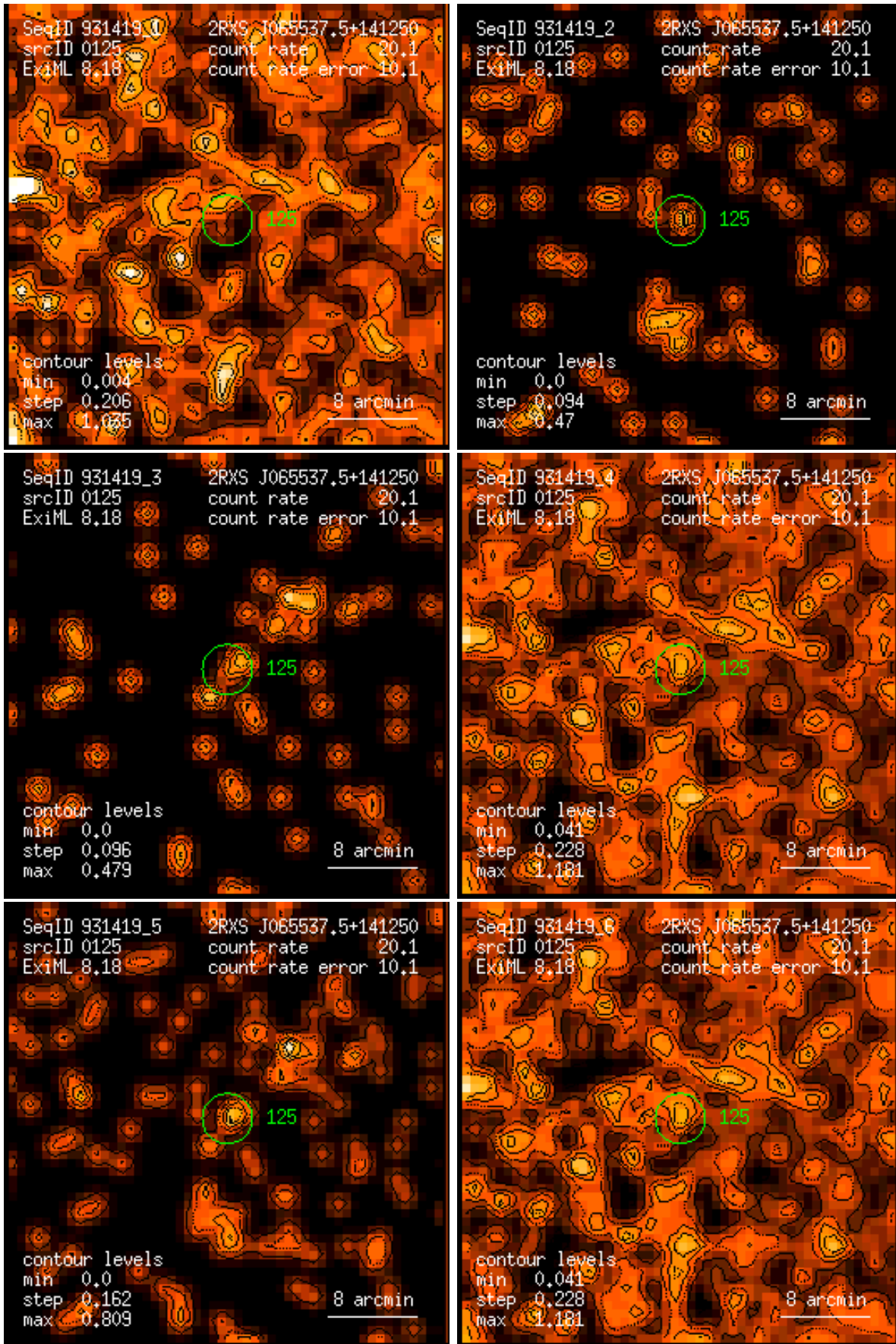
Figure 125: RASS 931419: detection 0125: band rate images, Gaussian filter: (1) PSPC channels 11 – 41, (2) 52 – 90, (3) 91 – 201, (4) 11 – 235, (5) 52 – 201, (6) 11 – 201. Broad band rates in counts/ks. Band rate contour levels in counts/ks/arcmin 2 .
