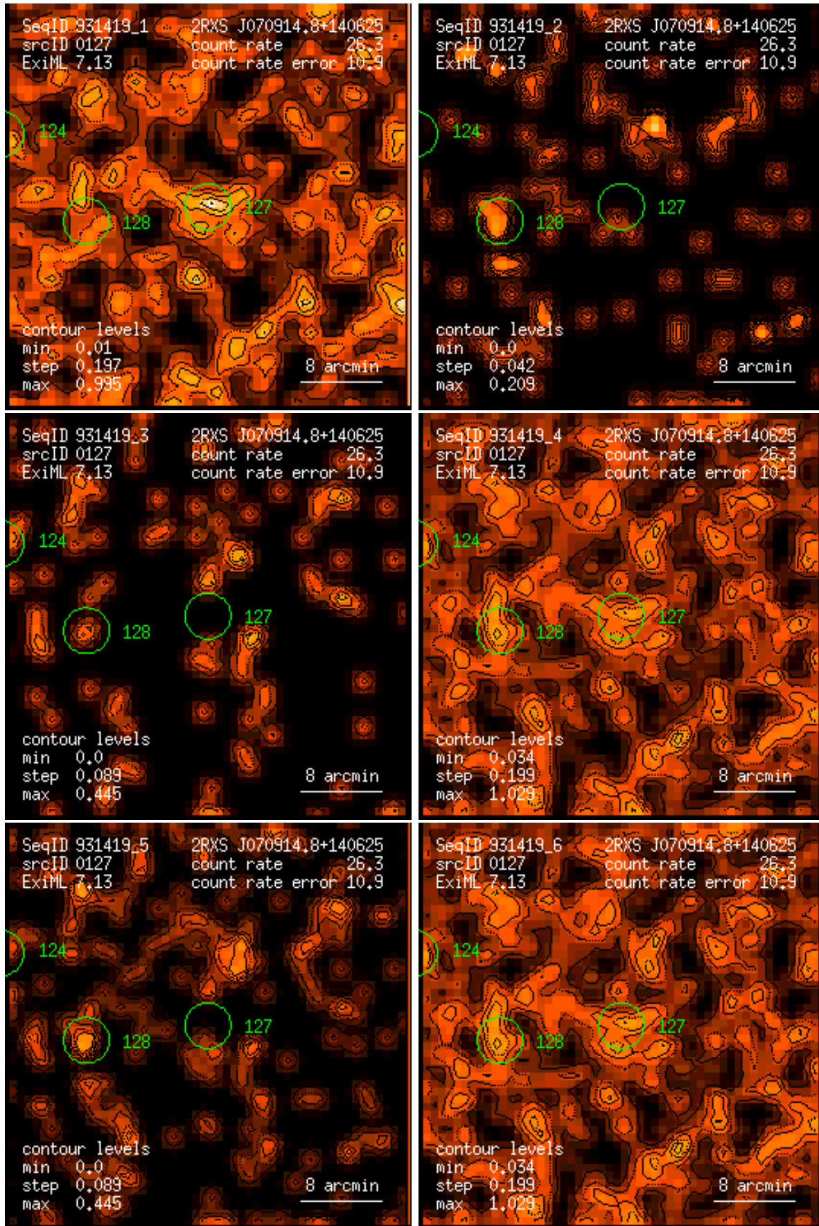
Figure 127: RASS 931419: detection 0127: band rate images, Gaussian filter: (1) PSPC channels 11 – 41, (2) 52 – 90, (3) 91 – 201, (4) 11 – 235, (5) 52 – 201, (6) 11 – 201. Broad band rates in counts/ks. Band rate contour levels in counts/ks/arcmin 2 .
