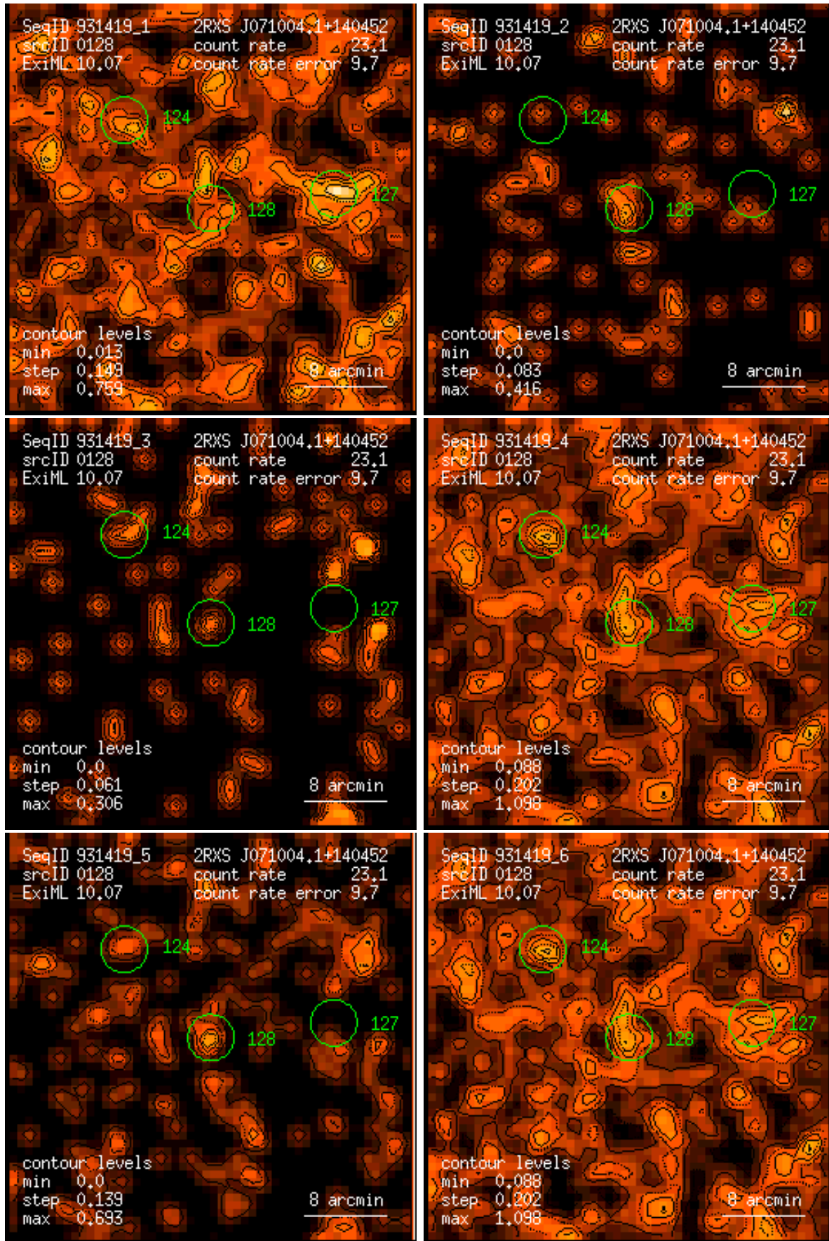
Figure 128: RASS 931419: detection 0128: band rate images, Gaussian filter: (1) PSPC channels 11 – 41, (2) 52 – 90, (3) 91 – 201, (4) 11 – 235, (5) 52 – 201, (6) 11 – 201. Broad band rates in counts/ks. Band rate contour levels in counts/ks/arcmin 2 .
