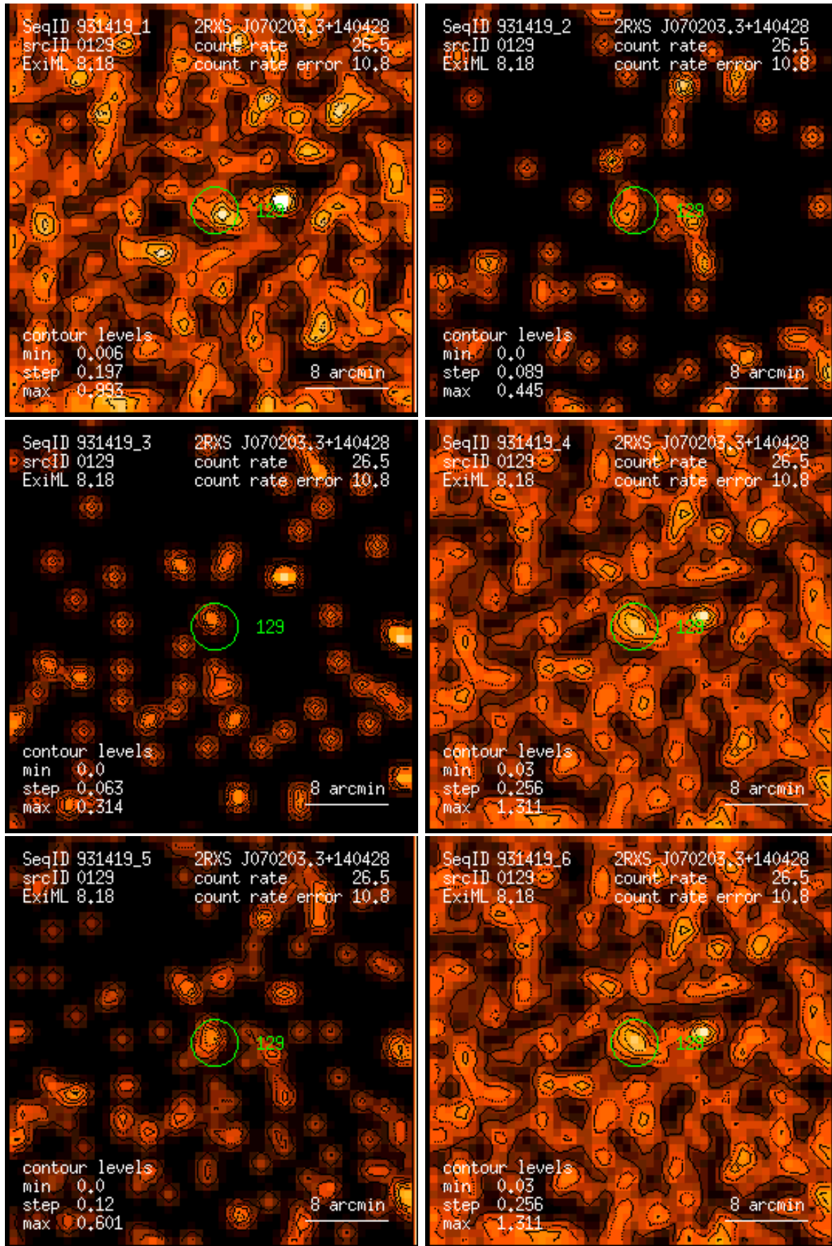
Figure 129: RASS 931419: detection 0129: band rate images, Gaussian filter: (1) PSPC channels 11 – 41, (2) 52 – 90, (3) 91 – 201, (4) 11 – 235, (5) 52 – 201, (6) 11 – 201. Broad band rates in counts/ks. Band rate contour levels in counts/ks/arcmin 2 .
