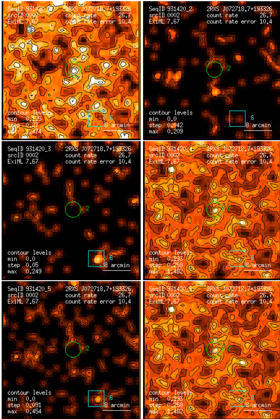
Figure 2: RASS 931420: detection 0002: band rate images, Gaussian filter: (1) PSPC channels 11 – 41, (2) 52 – 90, (3) 91 – 201, (4) 11 – 235, (5) 52 – 201, (6) 11 – 201. Broad band rates in counts/ks. Band rate contour levels in counts/ks/arcmin 2 .
