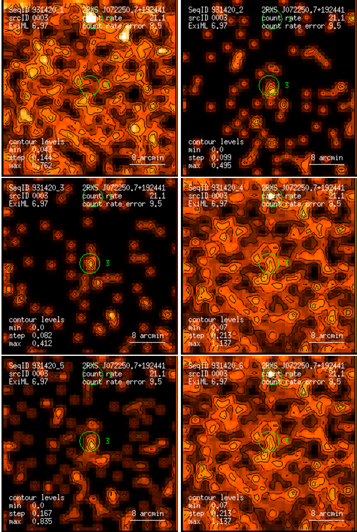
Figure 3: RASS 931420: detection 0003: band rate images, Gaussian filter: (1) PSPC channels 11 – 41, (2) 52 – 90, (3) 91 – 201, (4) 11 – 235, (5) 52 – 201, (6) 11 – 201. Broad band rates in counts/ks. Band rate contour levels in counts/ks/arcmin 2 .
