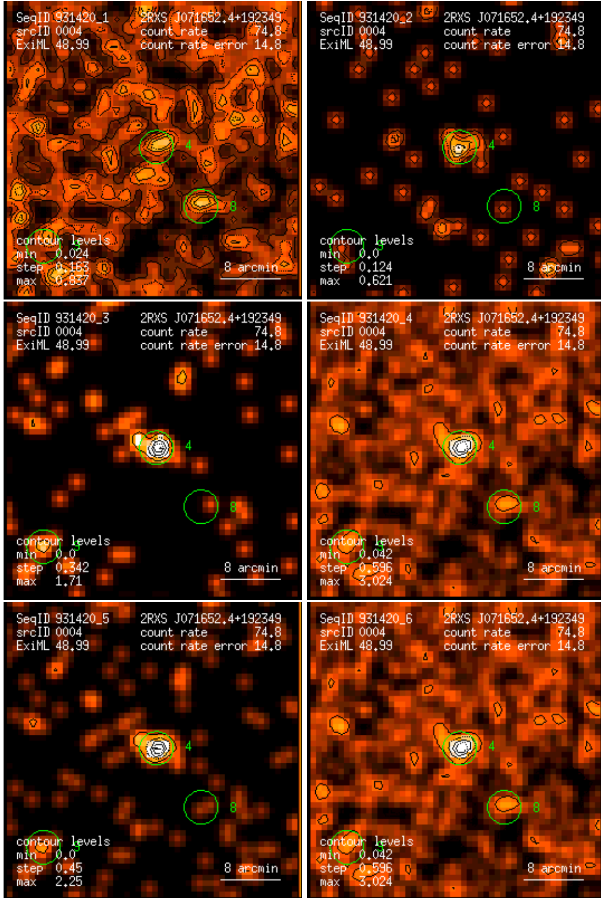
Figure 4: RASS 931420: detection 0004: band rate images, Gaussian filter: (1) PSPC channels 11 – 41, (2) 52 – 90, (3) 91 – 201, (4) 11 – 235, (5) 52 – 201, (6) 11 – 201. Broad band rates in counts/ks. Band rate contour levels in counts/ks/arcmin 2 .
