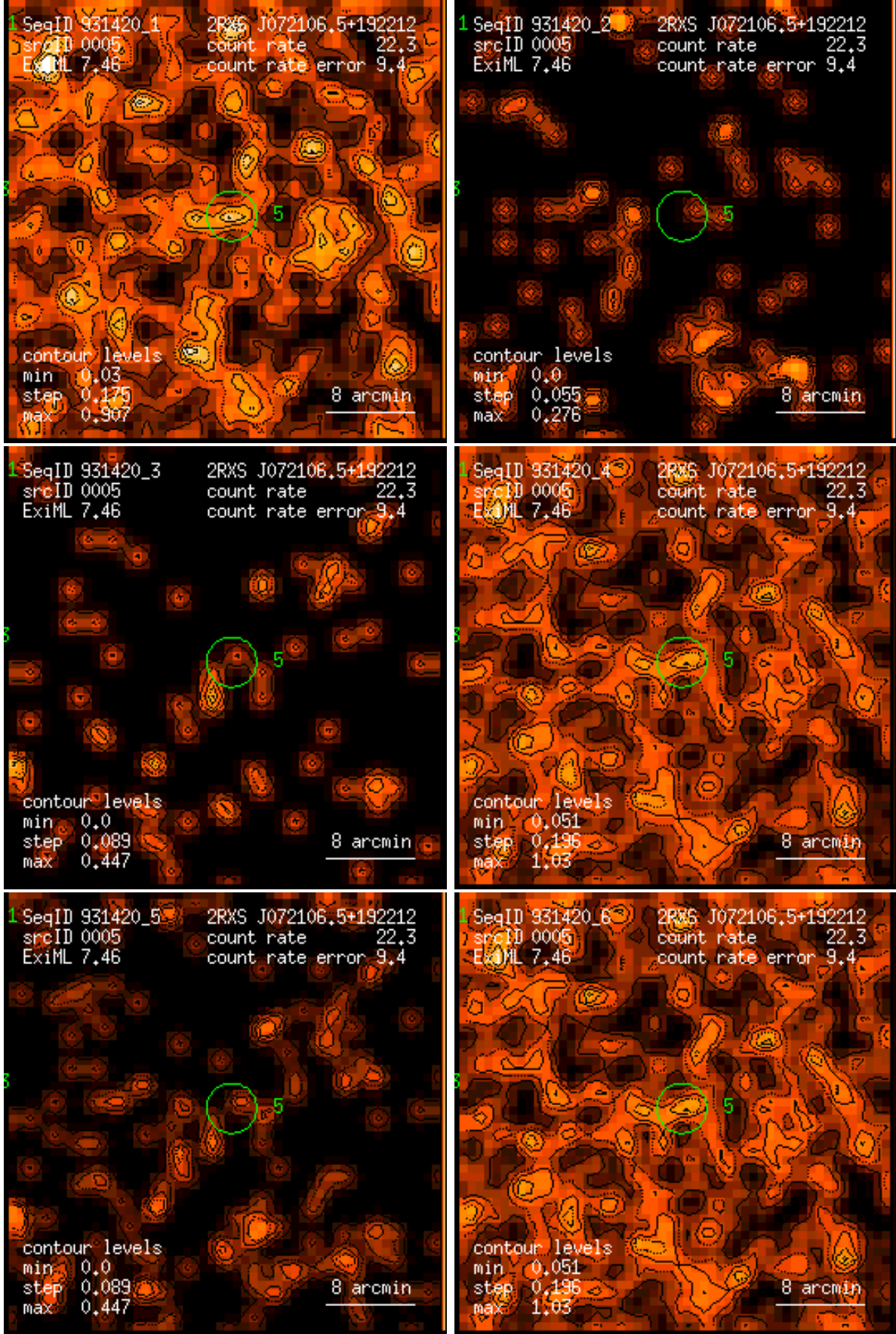
Figure 5: RASS 931420: detection 0005: band rate images, Gaussian filter: (1) PSPC channels 11 – 41, (2) 52 – 90, (3) 91 – 201, (4) 11 – 235, (5) 52 – 201, (6) 11 – 201. Broad band rates in counts/ks. Band rate contour levels in counts/ks/arcmin 2 .
