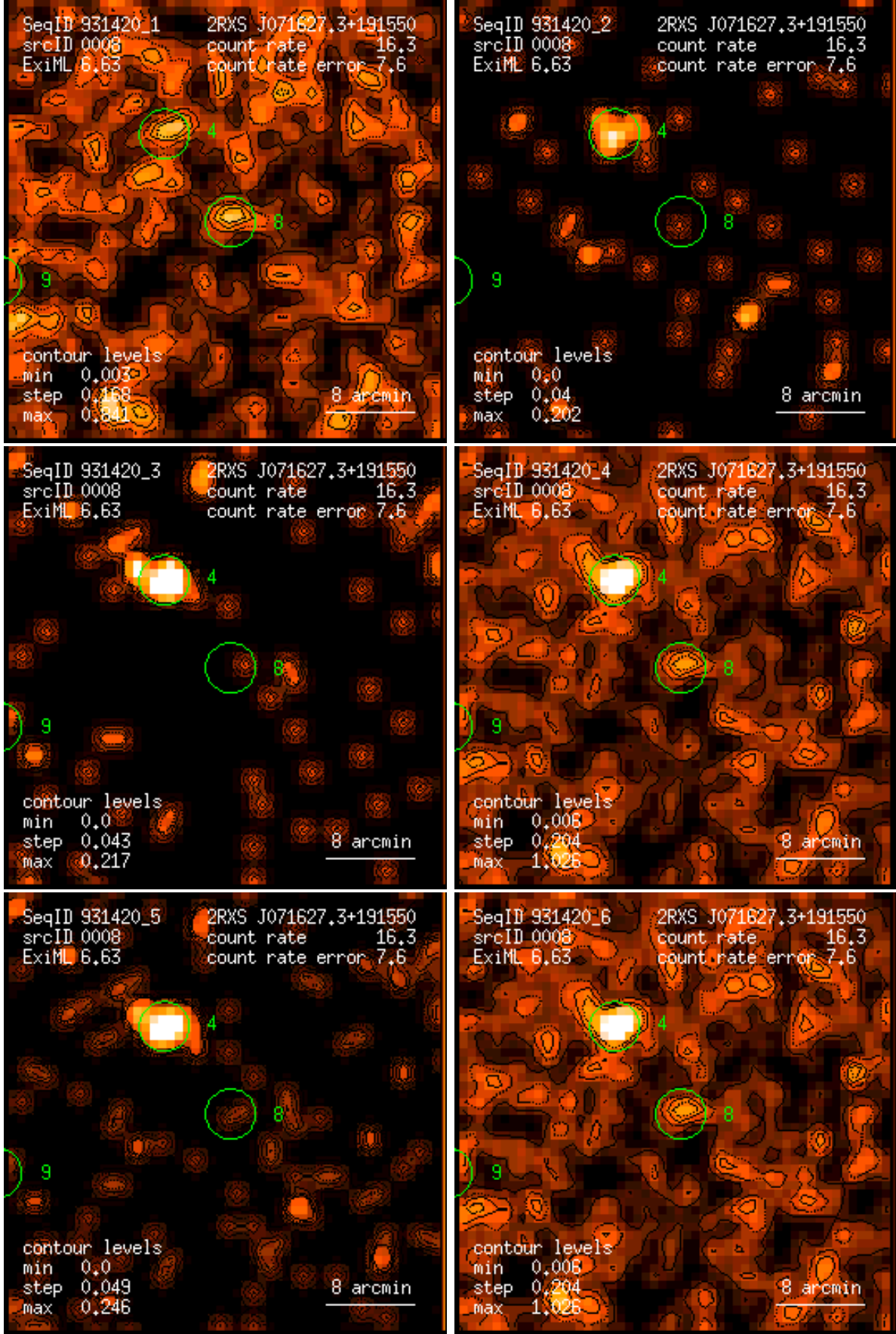
Figure 8: RASS 931420: detection 0008: band rate images, Gaussian filter: (1) PSPC channels 11 – 41, (2) 52 – 90, (3) 91 – 201, (4) 11 – 235, (5) 52 – 201, (6) 11 – 201. Broad band rates in counts/ks. Band rate contour levels in counts/ks/arcmin 2 .
