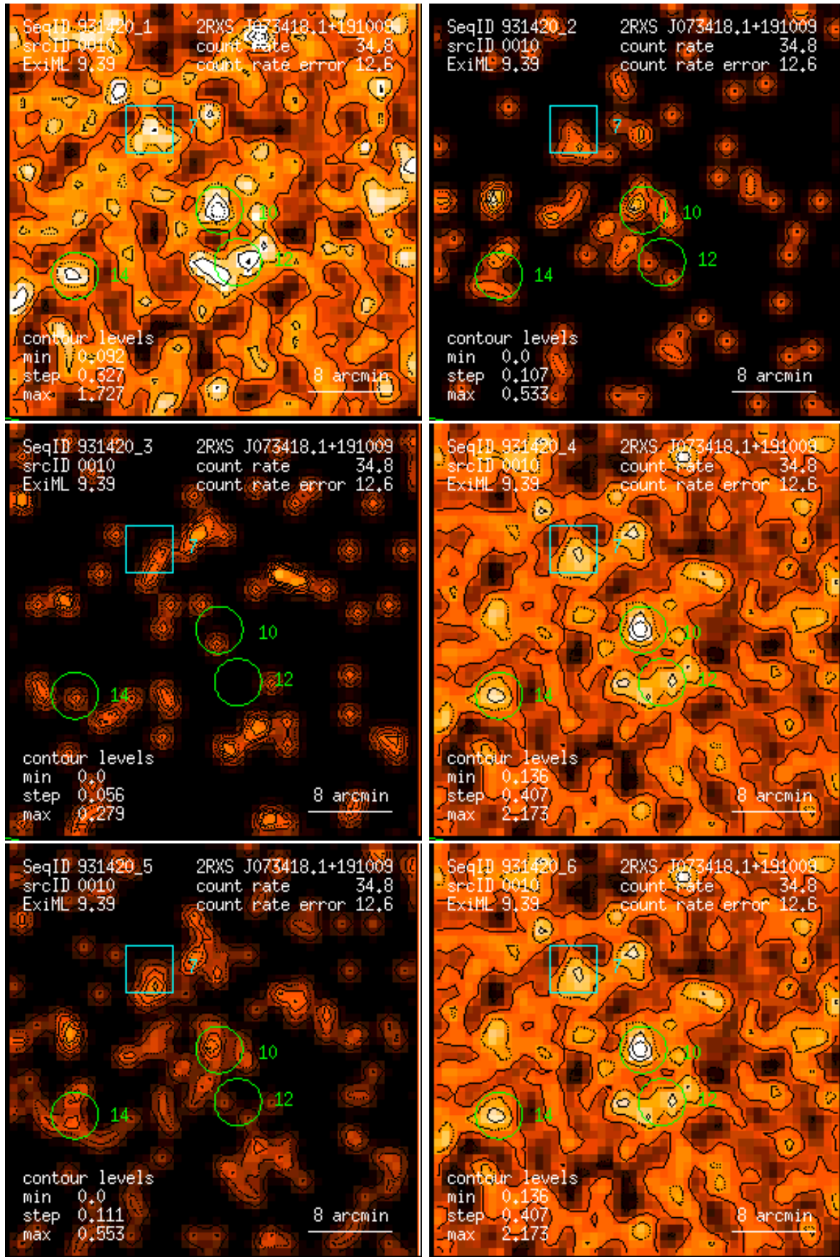
Figure 10: RASS 931420: detection 0010: band rate images, Gaussian filter: (1) PSPC channels 11 – 41, (2) 52 – 90, (3) 91 – 201, (4) 11 – 235, (5) 52 – 201, (6) 11 – 201. Broad band rates in counts/ks. Band rate contour levels in counts/ks/arcmin 2 .
