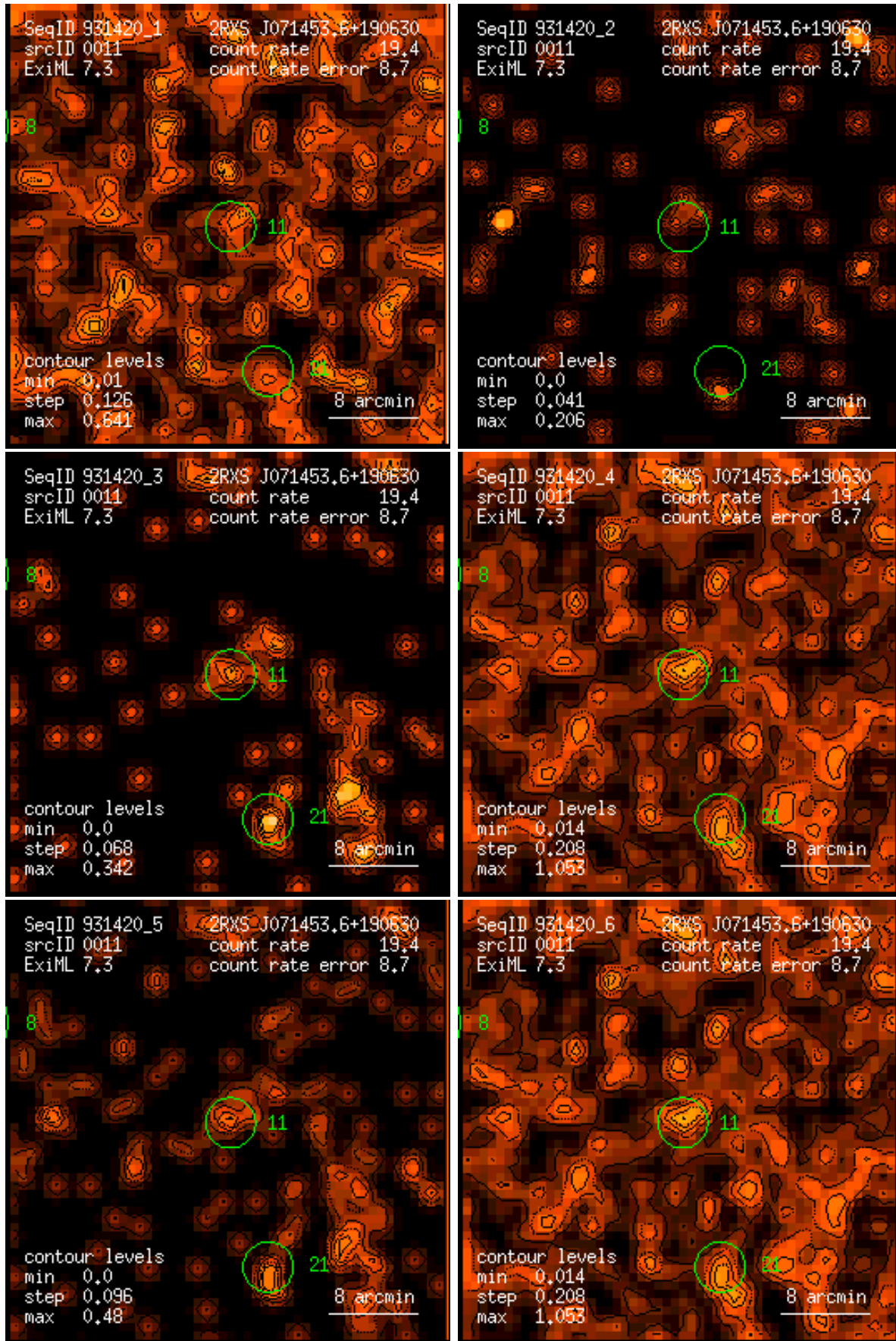
Figure 11: RASS 931420: detection 0011: band rate images, Gaussian filter: (1) PSPC channels 11 – 41, (2) 52 – 90, (3) 91 – 201, (4) 11 – 235, (5) 52 – 201, (6) 11 – 201. Broad band rates in counts/ks. Band rate contour levels in counts/ks/arcmin 2 .
