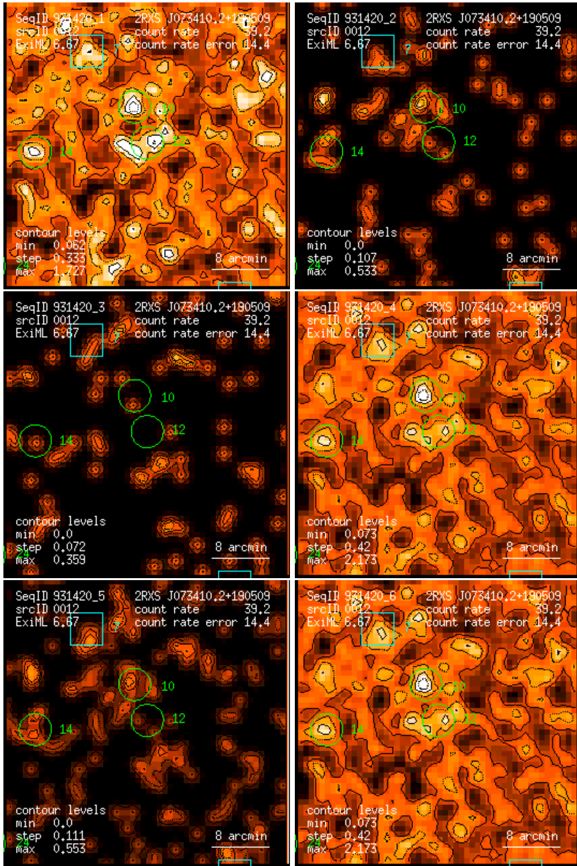
Figure 12: RASS 931420: detection 0012: band rate images, Gaussian filter: (1) PSPC channels 11 – 41, (2) 52 – 90, (3) 91 – 201, (4) 11 – 235, (5) 52 – 201, (6) 11 – 201. Broad band rates in counts/ks. Band rate contour levels in counts/ks/arcmin 2 .
