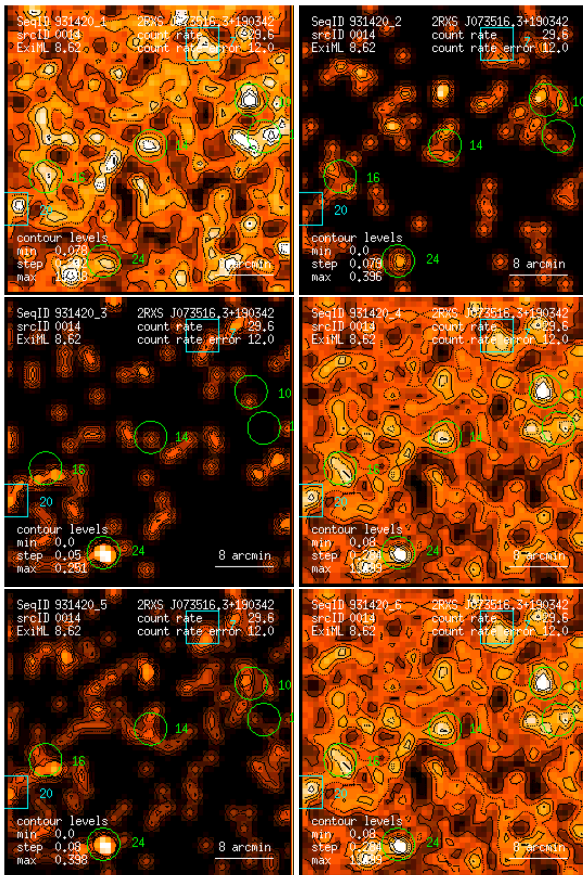
Figure 14: RASS 931420: detection 0014: band rate images, Gaussian filter: (1) PSPC channels 11 – 41, (2) 52 – 90, (3) 91 – 201, (4) 11 – 235, (5) 52 – 201, (6) 11 – 201. Broad band rates in counts/ks. Band rate contour levels in counts/ks/arcmin 2 .
