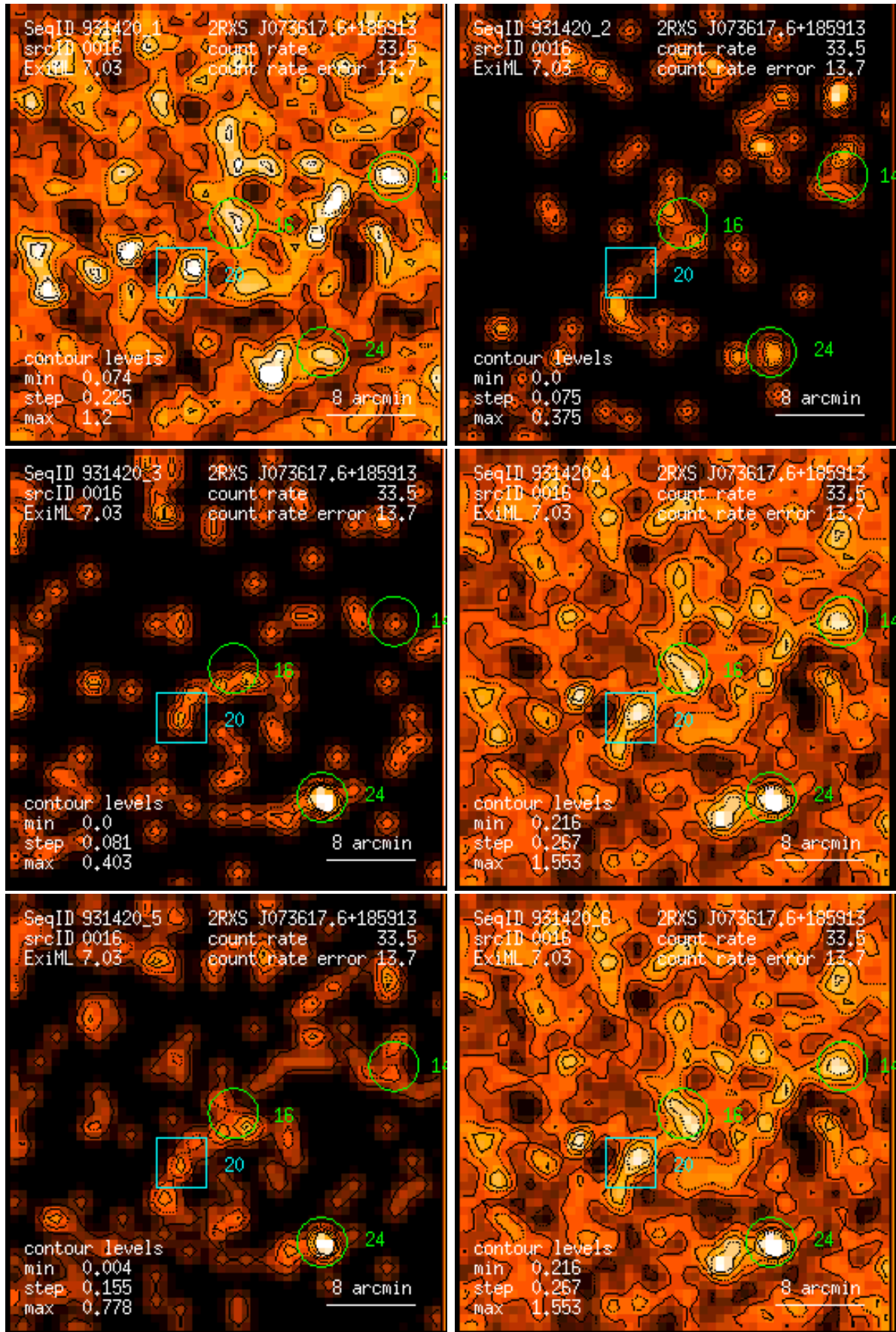
Figure 16: RASS 931420: detection 0016: band rate images, Gaussian filter: (1) PSPC channels 11 – 41, (2) 52 – 90, (3) 91 – 201, (4) 11 – 235, (5) 52 – 201, (6) 11 – 201. Broad band rates in counts/ks. Band rate contour levels in counts/ks/arcmin 2 .
