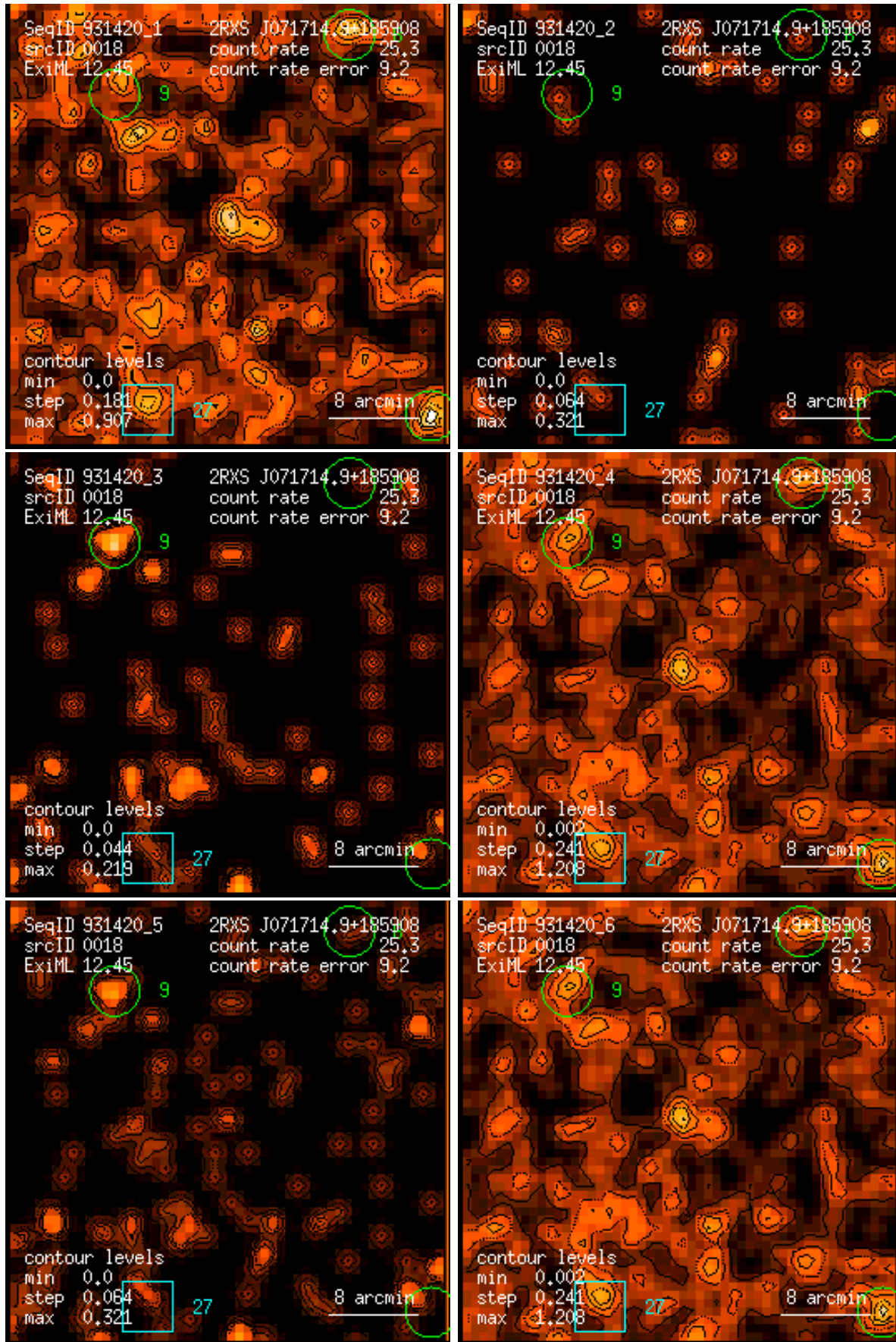
Figure 18: RASS 931420: detection 0018: band rate images, Gaussian filter: (1) PSPC channels 11 – 41, (2) 52 – 90, (3) 91 – 201, (4) 11 – 235, (5) 52 – 201, (6) 11 – 201. Broad band rates in counts/ks. Band rate contour levels in counts/ks/arcmin 2 .
