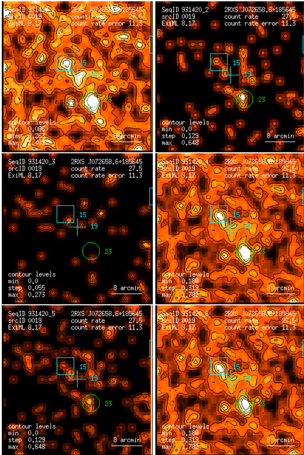
Figure 19: RASS 931420: detection 0019: band rate images, Gaussian filter: (1) PSPC channels 11 – 41, (2) 52 – 90, (3) 91 – 201, (4) 11 – 235, (5) 52 – 201, (6) 11 – 201. Broad band rates in counts/ks. Band rate contour levels in counts/ks/arcmin 2 .
