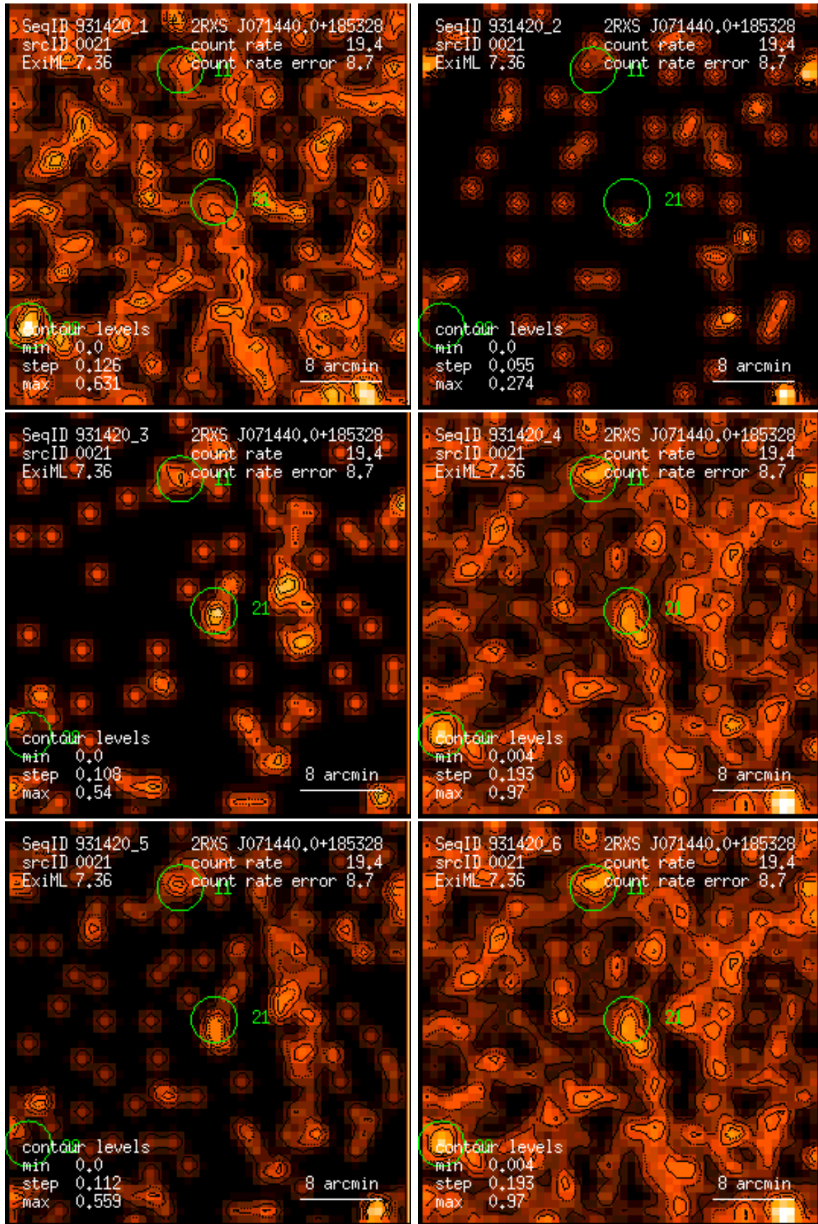
Figure 21: RASS 931420: detection 0021: band rate images, Gaussian filter: (1) PSPC channels 11 – 41, (2) 52 – 90, (3) 91 – 201, (4) 11 – 235, (5) 52 – 201, (6) 11 – 201. Broad band rates in counts/ks. Band rate contour levels in counts/ks/arcmin 2 .
