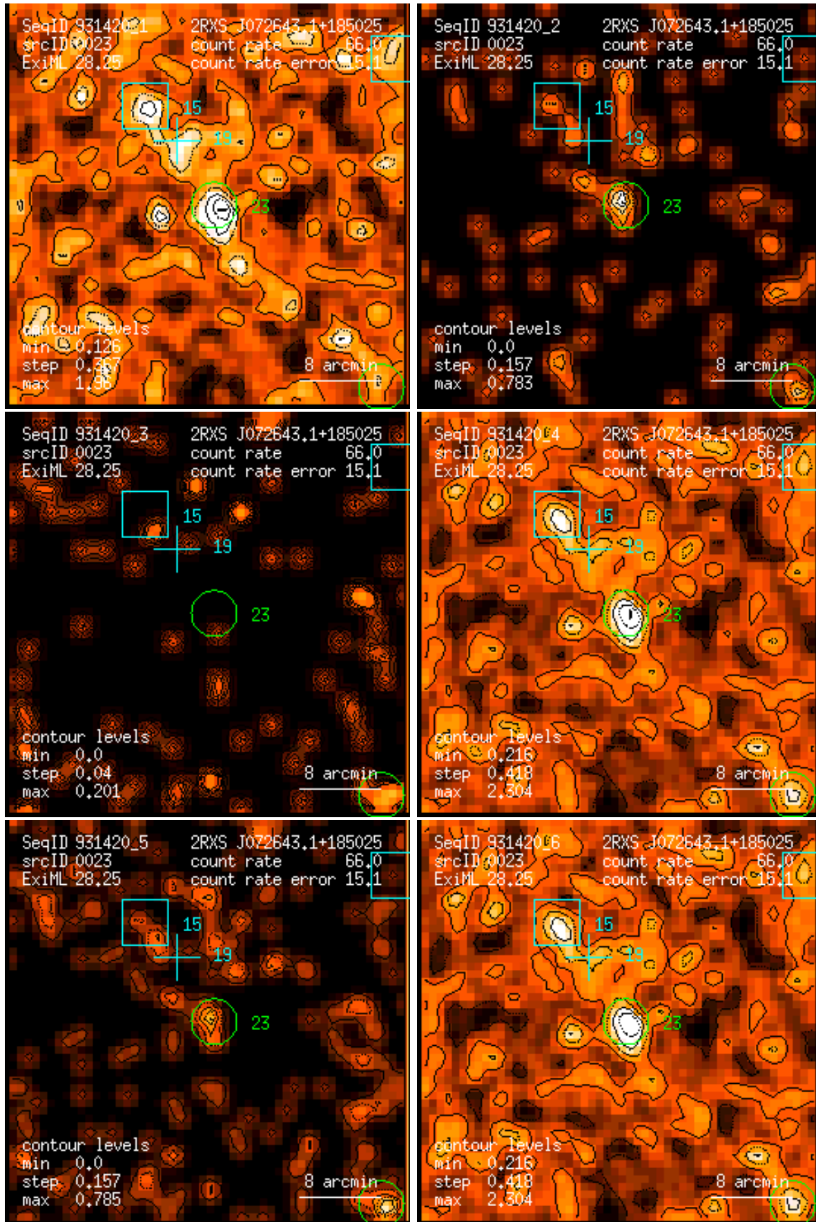
Figure 23: RASS 931420: detection 0023: band rate images, Gaussian filter: (1) PSPC channels 11 – 41, (2) 52 – 90, (3) 91 – 201, (4) 11 – 235, (5) 52 – 201, (6) 11 – 201. Broad band rates in counts/ks. Band rate contour levels in counts/ks/arcmin 2 .
