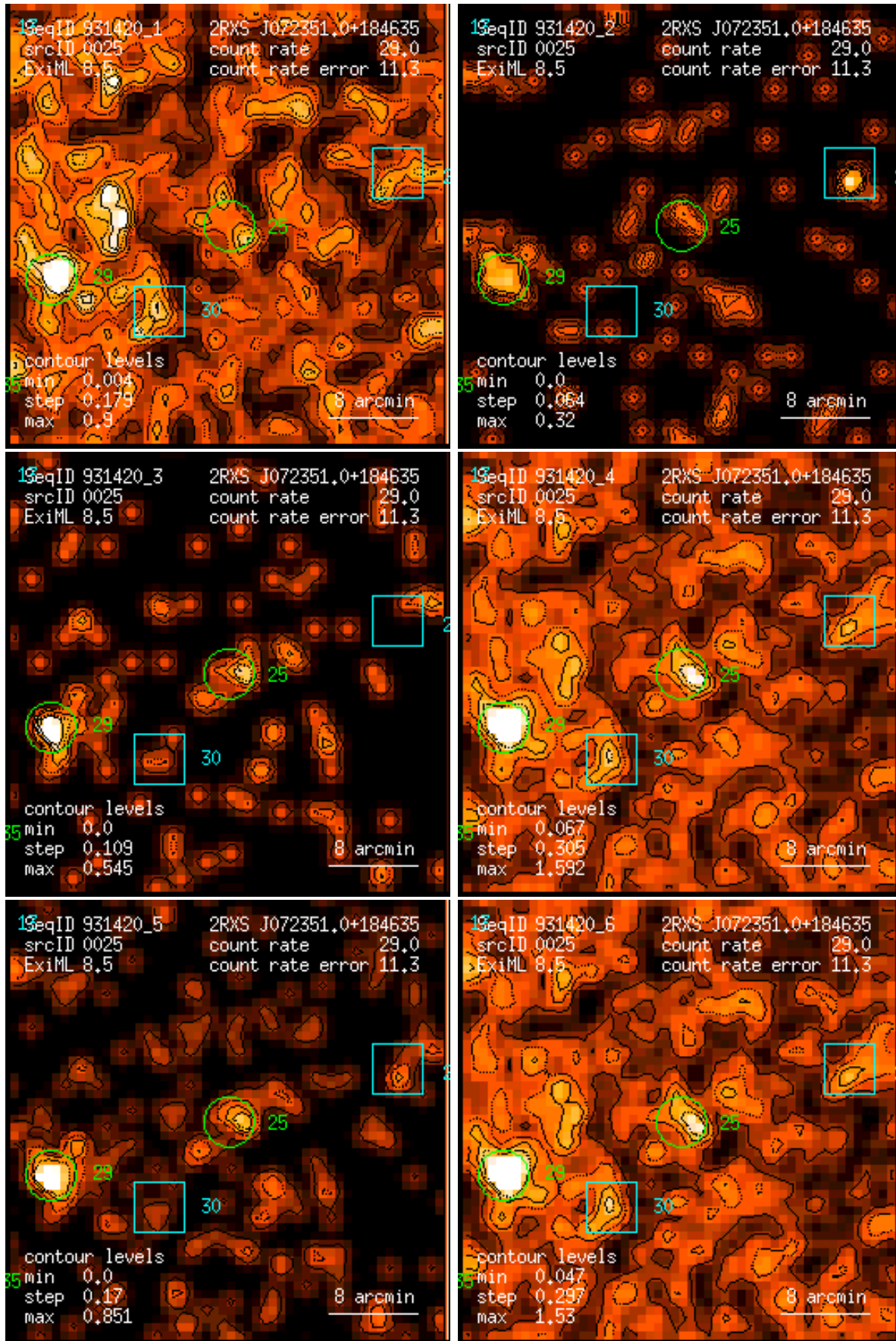
Figure 25: RASS 931420: detection 0025: band rate images, Gaussian filter: (1) PSPC channels 11 – 41, (2) 52 – 90, (3) 91 – 201, (4) 11 – 235, (5) 52 – 201, (6) 11 – 201. Broad band rates in counts/ks. Band rate contour levels in counts/ks/arcmin 2 .
