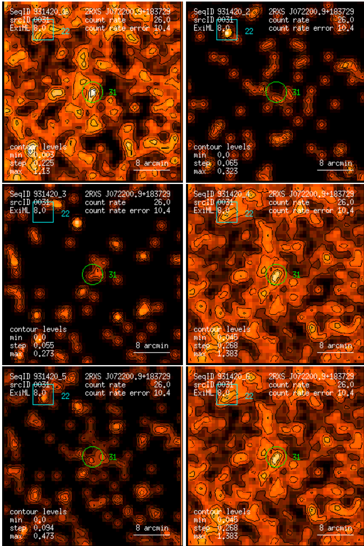
Figure 31: RASS 931420: detection 0031: band rate images, Gaussian filter: (1) PSPC channels 11 – 41, (2) 52 – 90, (3) 91 – 201, (4) 11 – 235, (5) 52 – 201, (6) 11 – 201. Broad band rates in counts/ks. Band rate contour levels in counts/ks/arcmin 2 .
