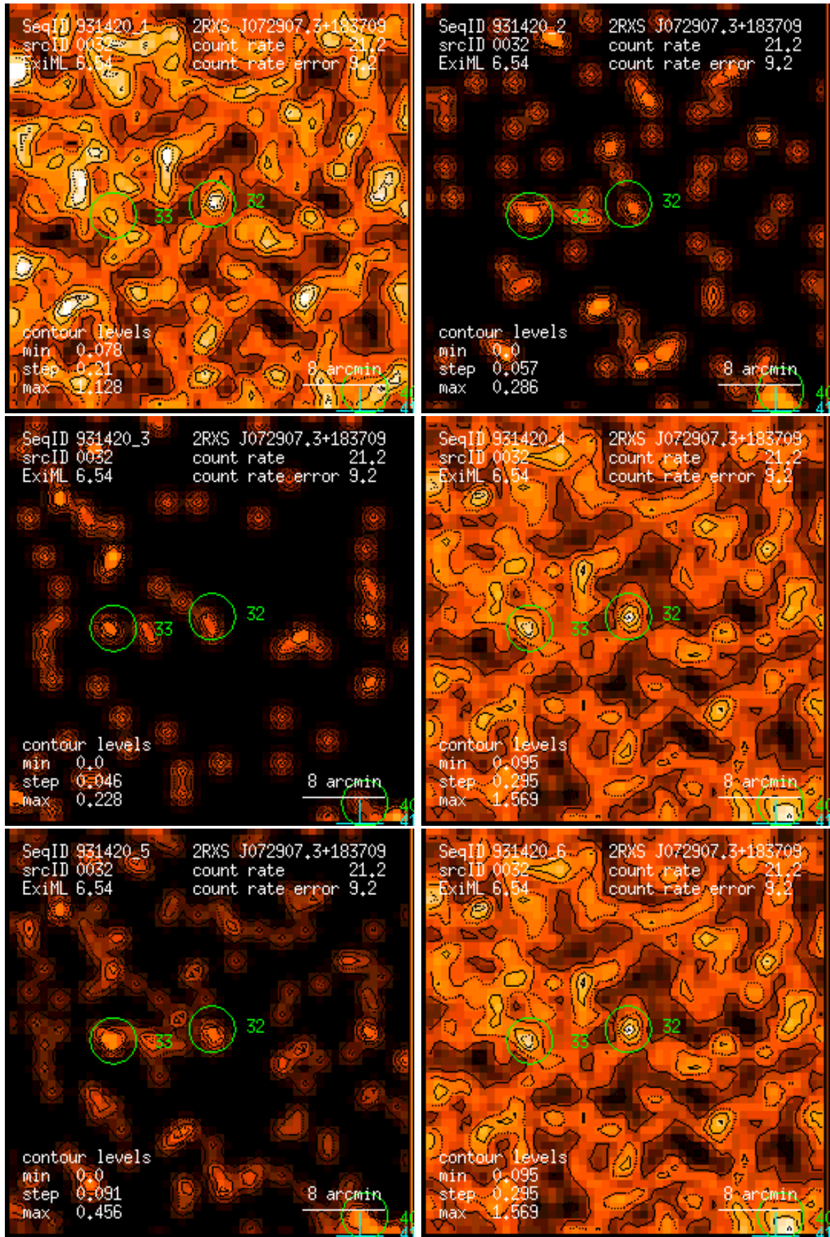
Figure 32: RASS 931420: detection 0032: band rate images, Gaussian filter: (1) PSPC channels 11 – 41, (2) 52 – 90, (3) 91 – 201, (4) 11 – 235, (5) 52 – 201, (6) 11 – 201. Broad band rates in counts/ks. Band rate contour levels in counts/ks/arcmin 2 .
