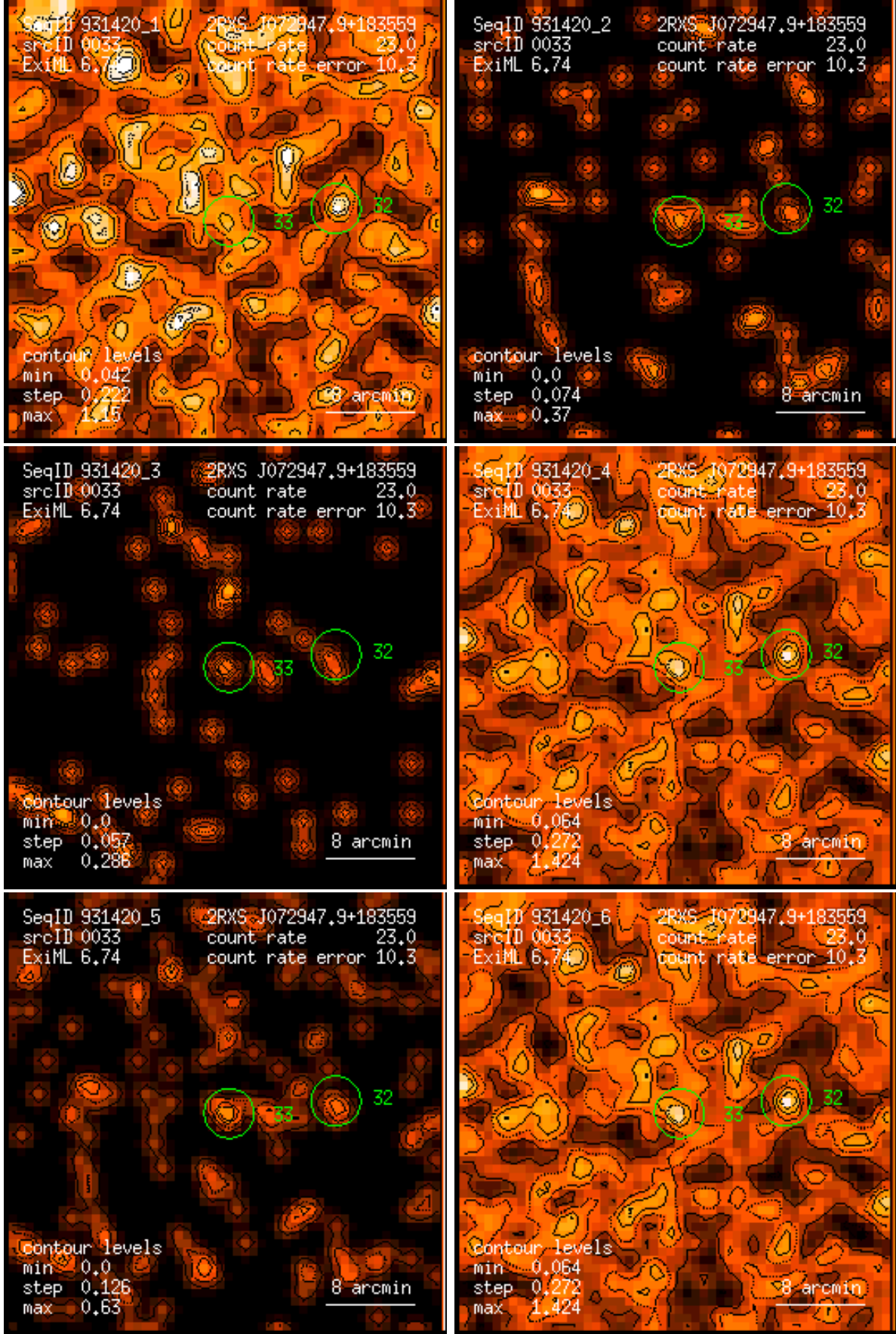
Figure 33: RASS 931420: detection 0033: band rate images, Gaussian filter: (1) PSPC channels 11 – 41, (2) 52 – 90, (3) 91 – 201, (4) 11 – 235, (5) 52 – 201, (6) 11 – 201. Broad band rates in counts/ks. Band rate contour levels in counts/ks/arcmin 2 .
