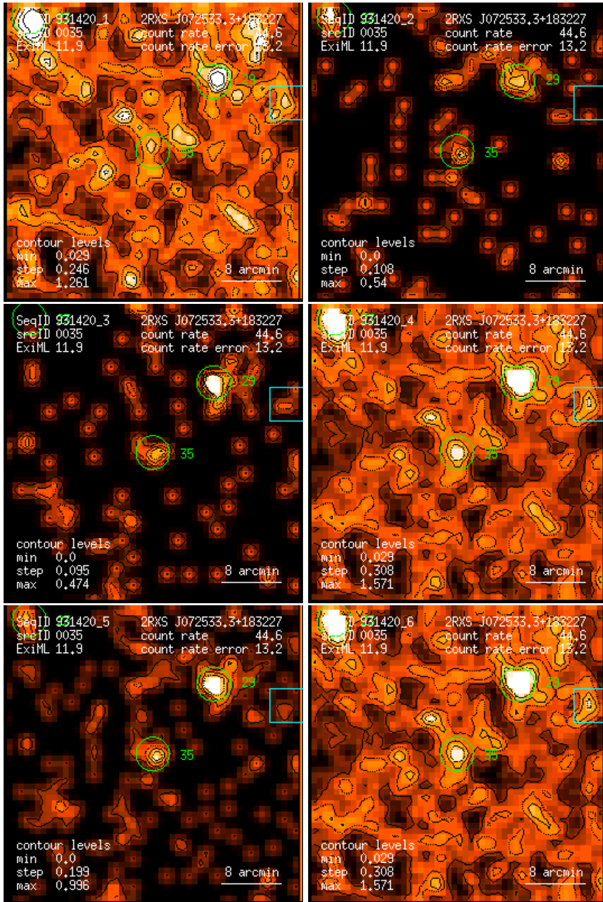
Figure 35: RASS 931420: detection 0035: band rate images, Gaussian filter: (1) PSPC channels 11 – 41, (2) 52 – 90, (3) 91 – 201, (4) 11 – 235, (5) 52 – 201, (6) 11 – 201. Broad band rates in counts/ks. Band rate contour levels in counts/ks/arcmin 2 .
