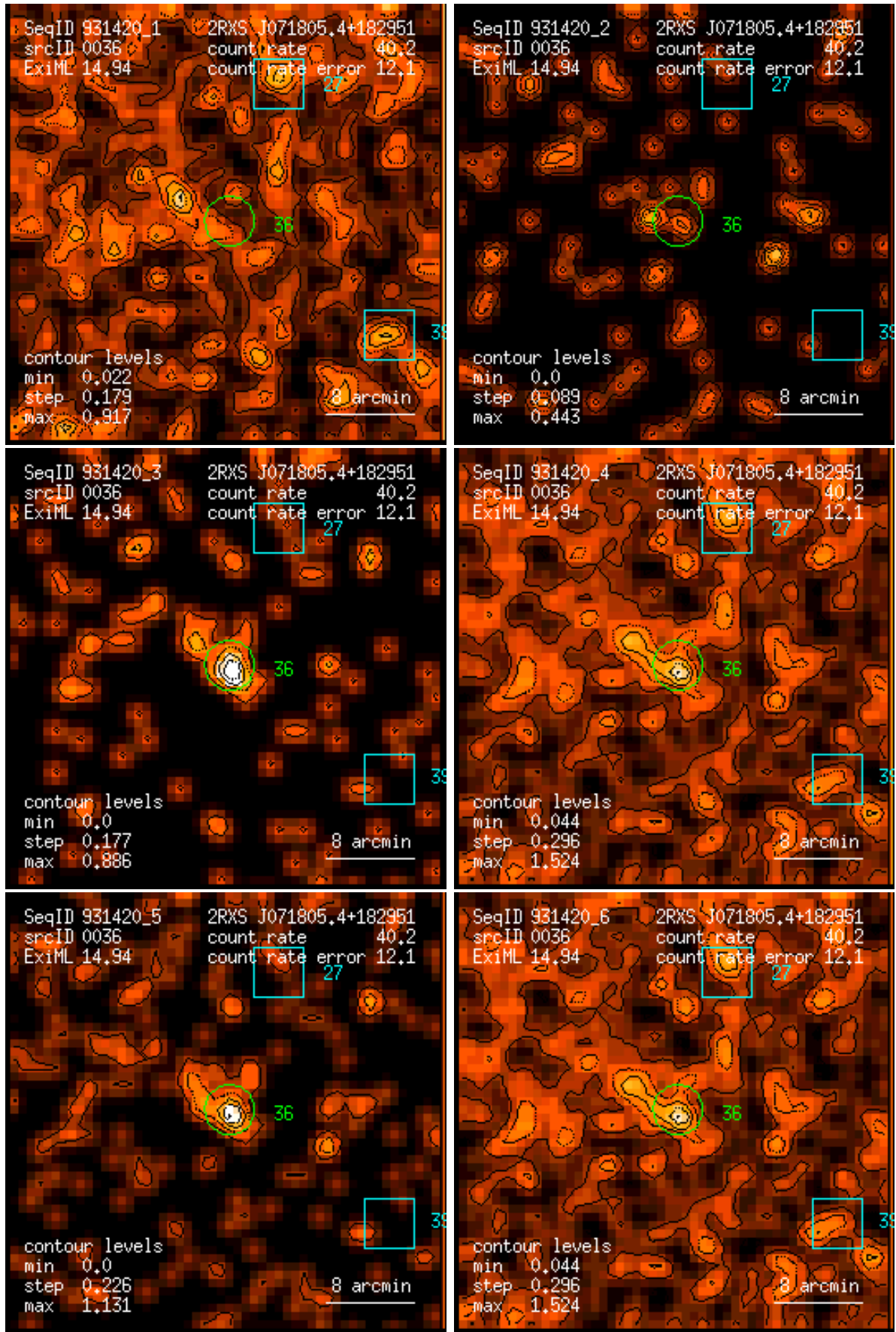
Figure 36: RASS 931420: detection 0036: band rate images, Gaussian filter: (1) PSPC channels 11 – 41, (2) 52 – 90, (3) 91 – 201, (4) 11 – 235, (5) 52 – 201, (6) 11 – 201. Broad band rates in counts/ks. Band rate contour levels in counts/ks/arcmin 2 .
