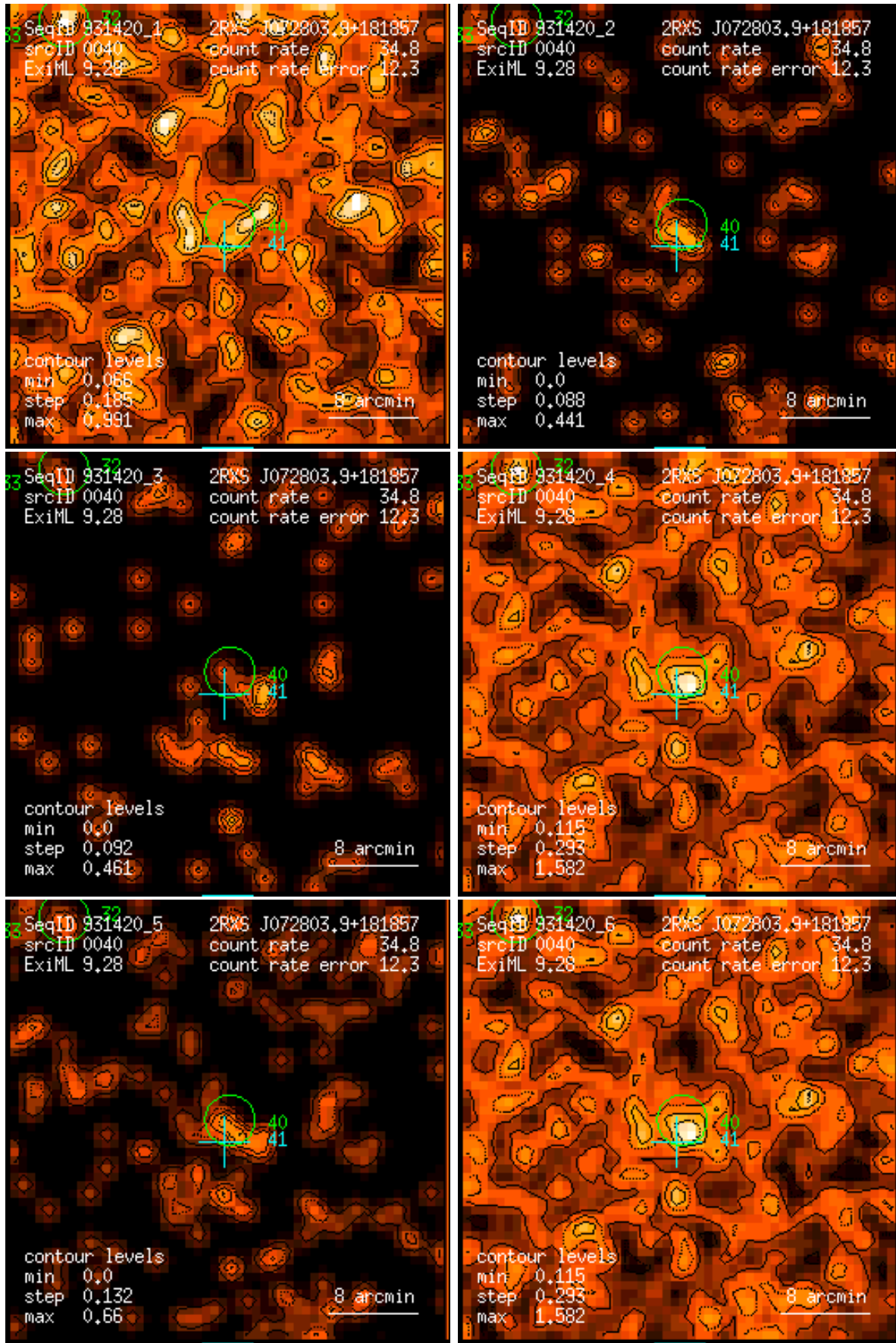
Figure 40: RASS 931420: detection 0040: band rate images, Gaussian filter: (1) PSPC channels 11 – 41, (2) 52 – 90, (3) 91 – 201, (4) 11 – 235, (5) 52 – 201, (6) 11 – 201. Broad band rates in counts/ks. Band rate contour levels in counts/ks/arcmin 2 .
