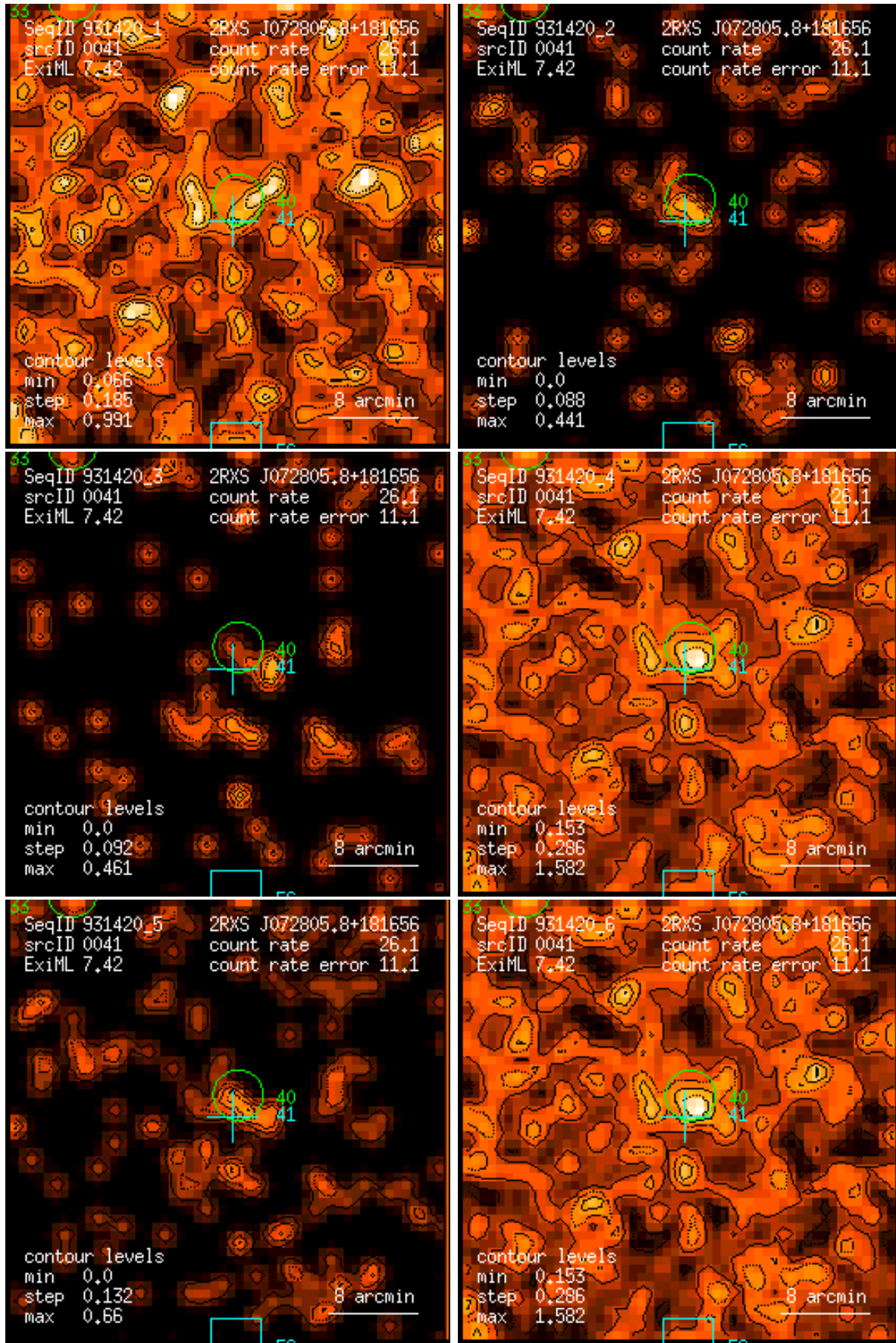
Figure 41: RASS 931420: detection 0041: band rate images, Gaussian filter: (1) PSPC channels 11 – 41, (2) 52 – 90, (3) 91 – 201, (4) 11 – 235, (5) 52 – 201, (6) 11 – 201. Broad band rates in counts/ks. Band rate contour levels in counts/ks/arcmin 2 .
