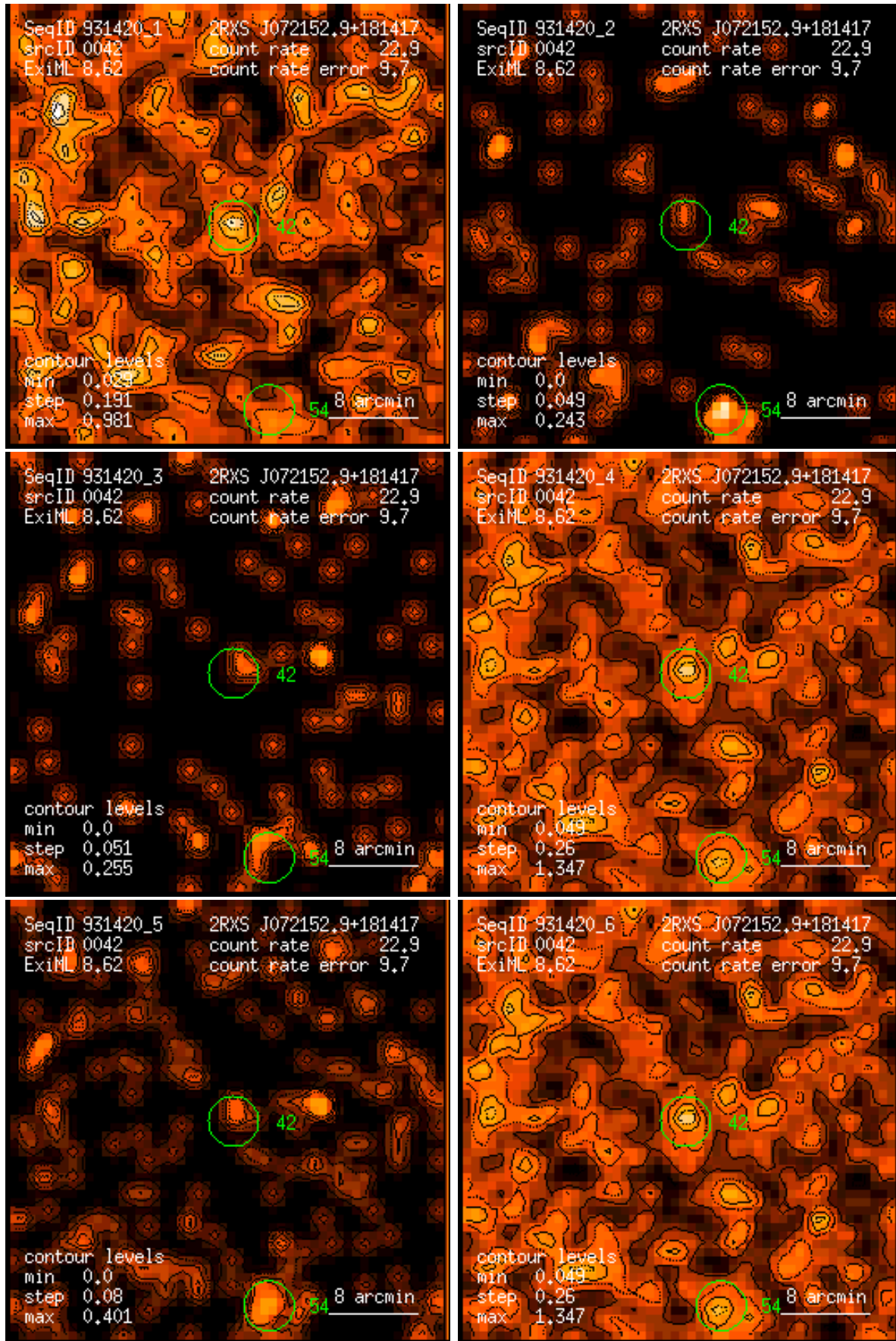
Figure 42: RASS 931420: detection 0042: band rate images, Gaussian filter: (1) PSPC channels 11 – 41, (2) 52 – 90, (3) 91 – 201, (4) 11 – 235, (5) 52 – 201, (6) 11 – 201. Broad band rates in counts/ks. Band rate contour levels in counts/ks/arcmin 2 .
