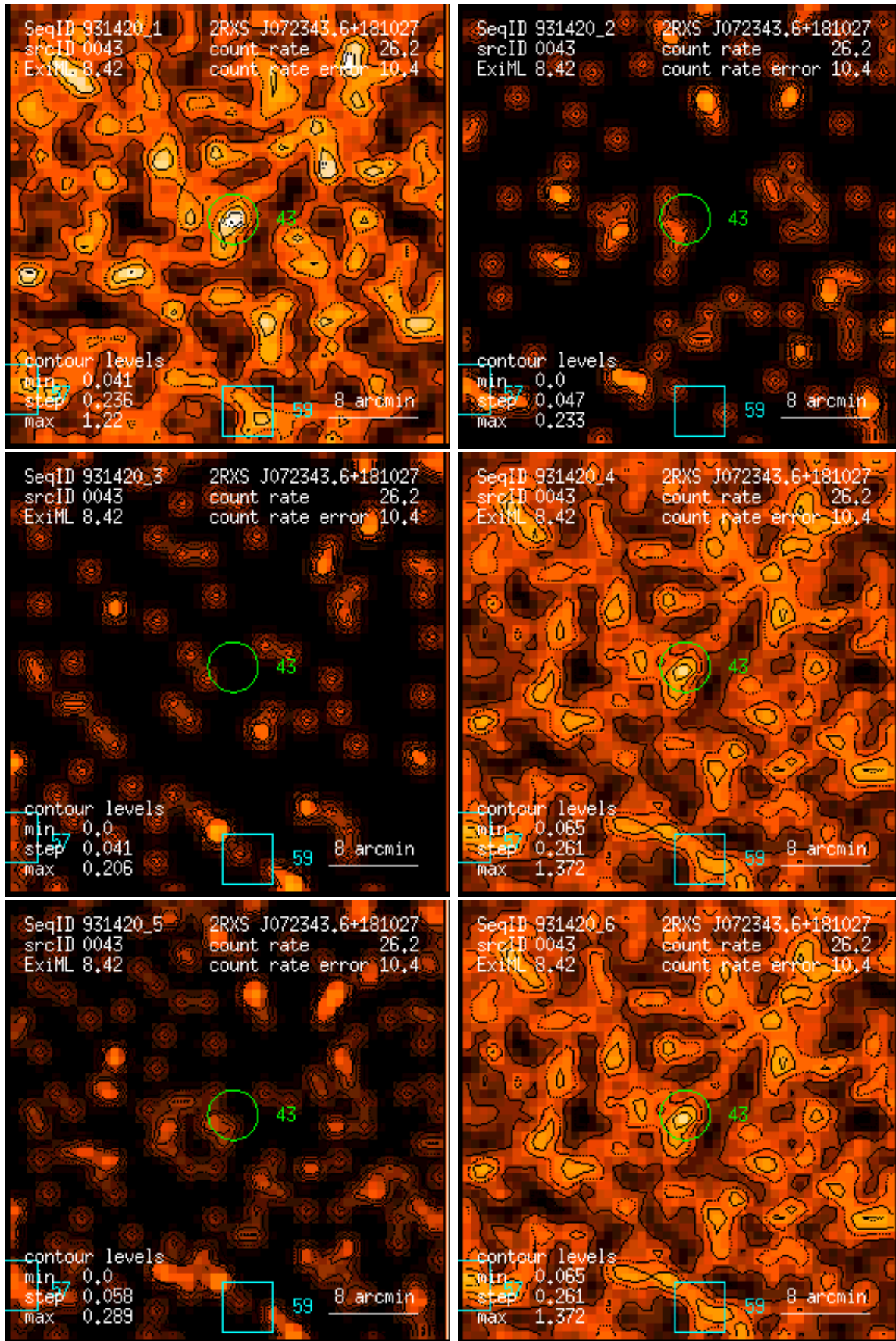
Figure 43: RASS 931420: detection 0043: band rate images, Gaussian filter: (1) PSPC channels 11 – 41, (2) 52 – 90, (3) 91 – 201, (4) 11 – 235, (5) 52 – 201, (6) 11 – 201. Broad band rates in counts/ks. Band rate contour levels in counts/ks/arcmin 2 .
