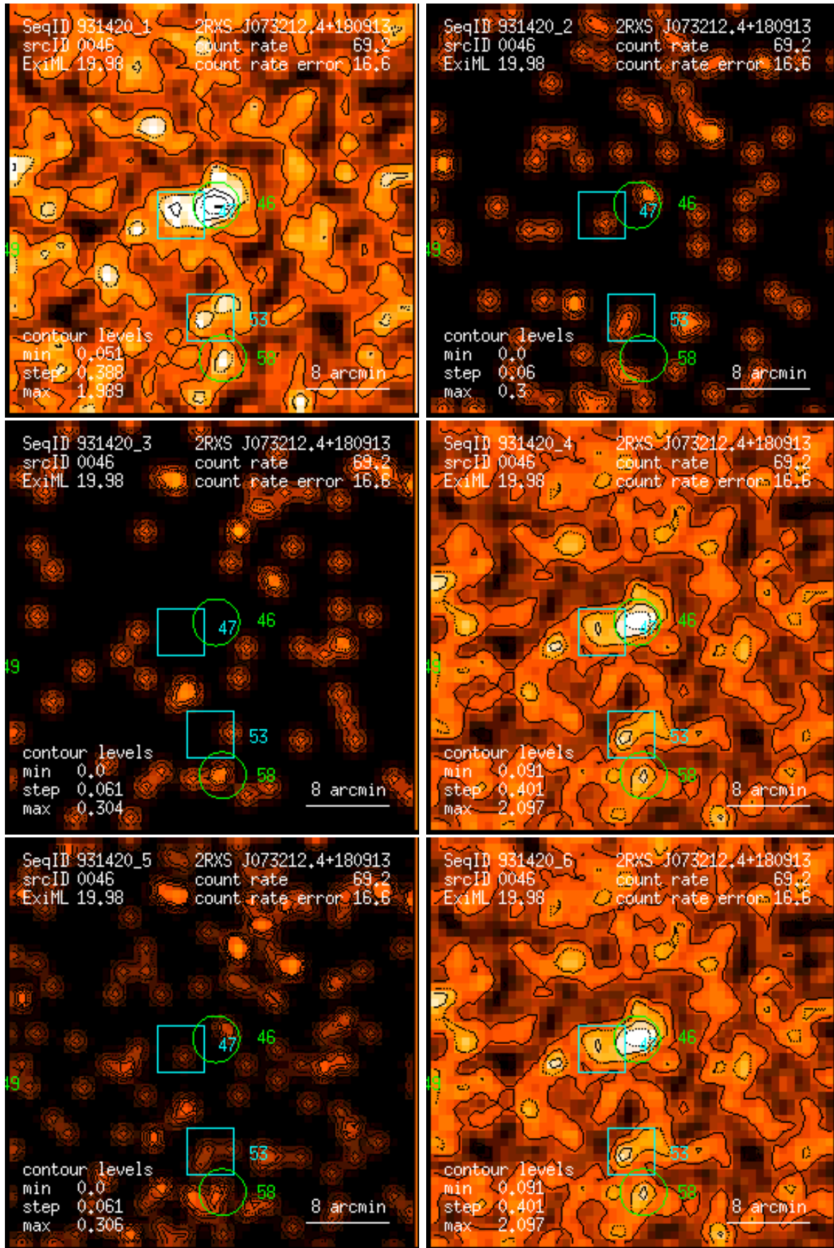
Figure 46: RASS 931420: detection 0046: band rate images, Gaussian filter: (1) PSPC channels 11 – 41, (2) 52 – 90, (3) 91 – 201, (4) 11 – 235, (5) 52 – 201, (6) 11 – 201. Broad band rates in counts/ks. Band rate contour levels in counts/ks/arcmin 2 .
