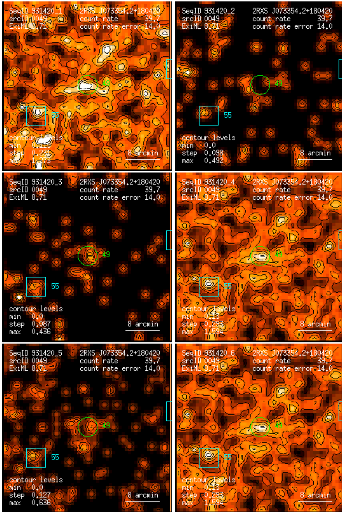
Figure 49: RASS 931420: detection 0049: band rate images, Gaussian filter: (1) PSPC channels 11 – 41, (2) 52 – 90, (3) 91 – 201, (4) 11 – 235, (5) 52 – 201, (6) 11 – 201. Broad band rates in counts/ks. Band rate contour levels in counts/ks/arcmin 2 .
