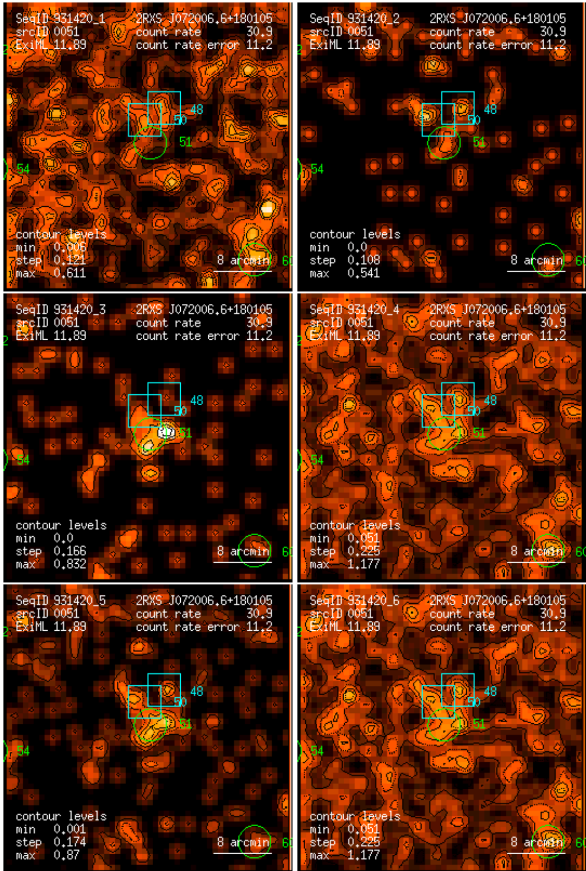
Figure 51: RASS 931420: detection 0051: band rate images, Gaussian filter: (1) PSPC channels 11 – 41, (2) 52 – 90, (3) 91 – 201, (4) 11 – 235, (5) 52 – 201, (6) 11 – 201. Broad band rates in counts/ks. Band rate contour levels in counts/ks/arcmin 2 .
