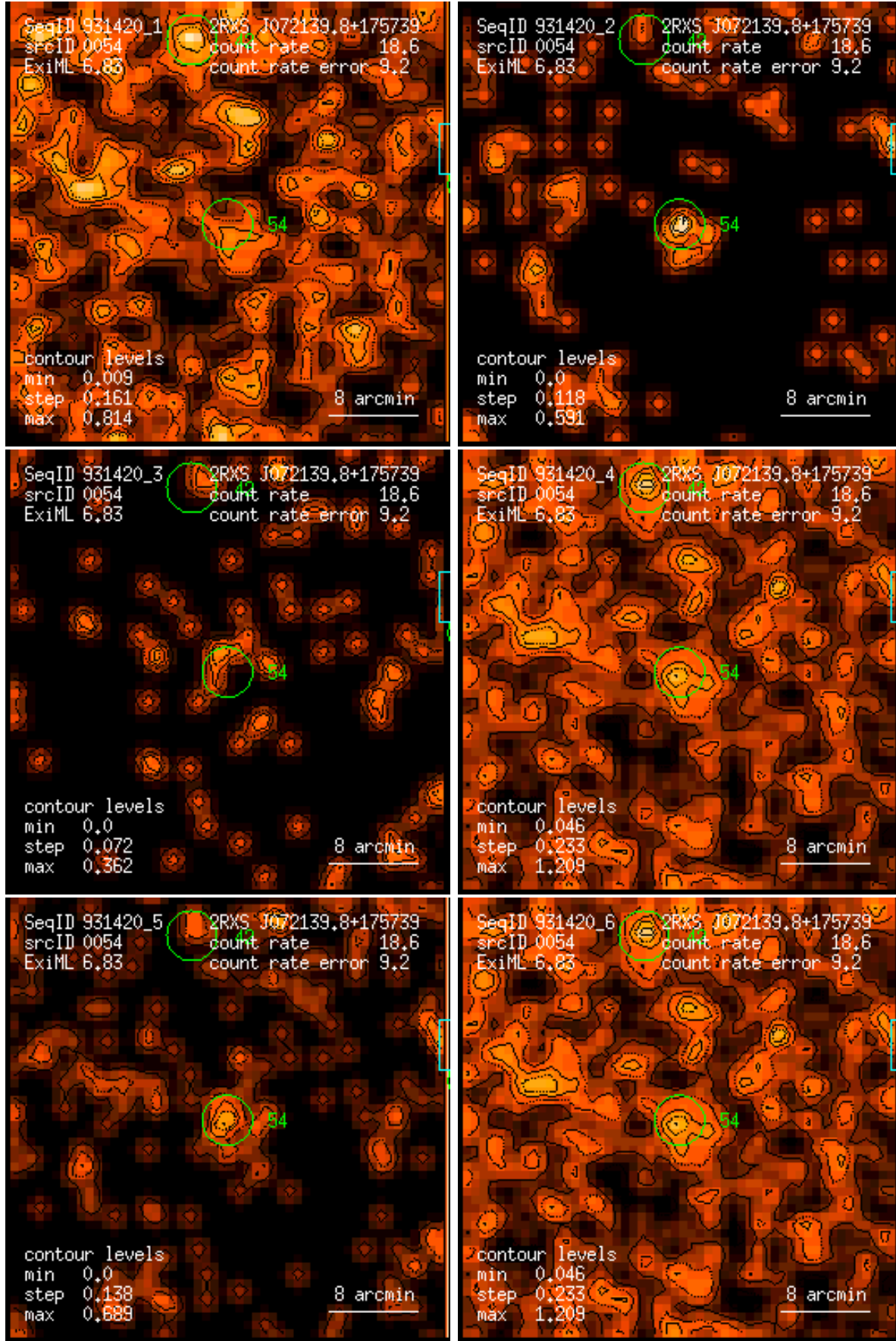
Figure 54: RASS 931420: detection 0054: band rate images, Gaussian filter: (1) PSPC channels 11 – 41, (2) 52 – 90, (3) 91 – 201, (4) 11 – 235, (5) 52 – 201, (6) 11 – 201. Broad band rates in counts/ks. Band rate contour levels in counts/ks/arcmin 2 .
