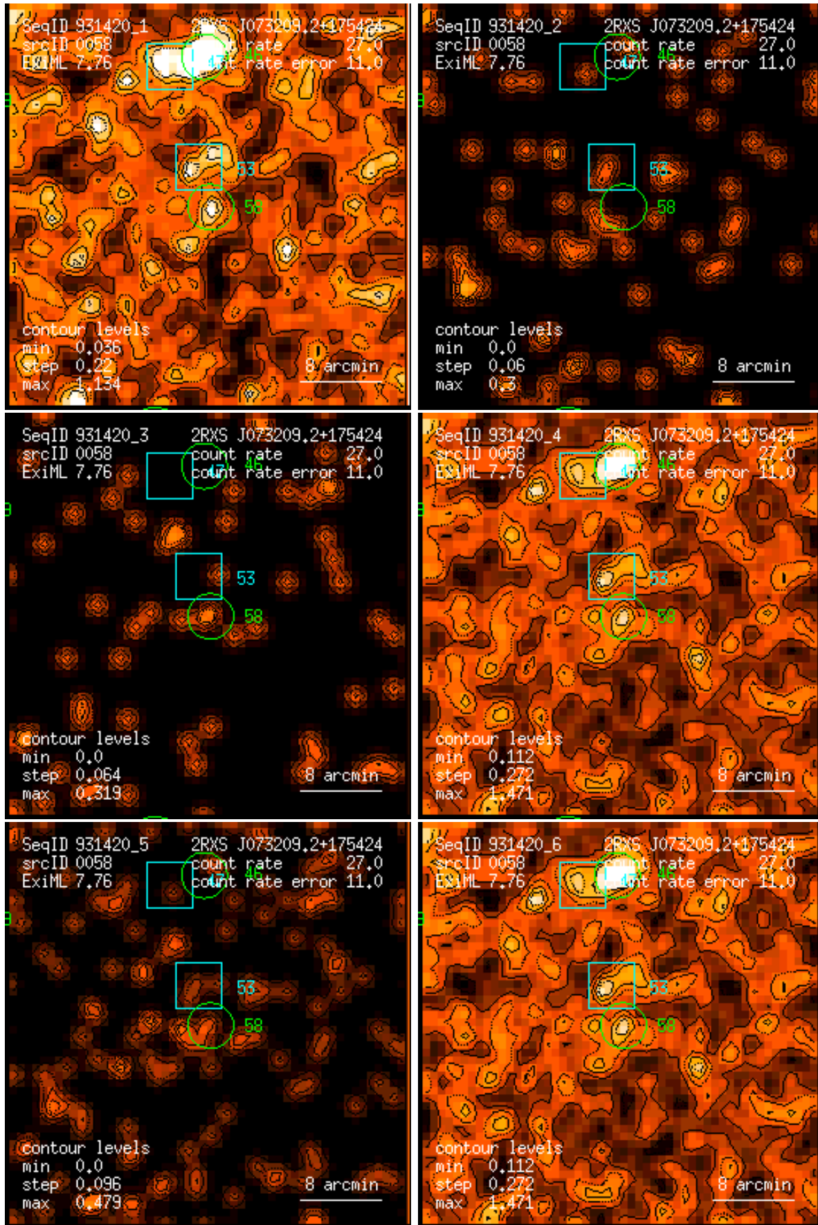
Figure 58: RASS 931420: detection 0058: band rate images, Gaussian filter: (1) PSPC channels 11 – 41, (2) 52 – 90, (3) 91 – 201, (4) 11 – 235, (5) 52 – 201, (6) 11 – 201. Broad band rates in counts/ks. Band rate contour levels in counts/ks/arcmin 2 .
