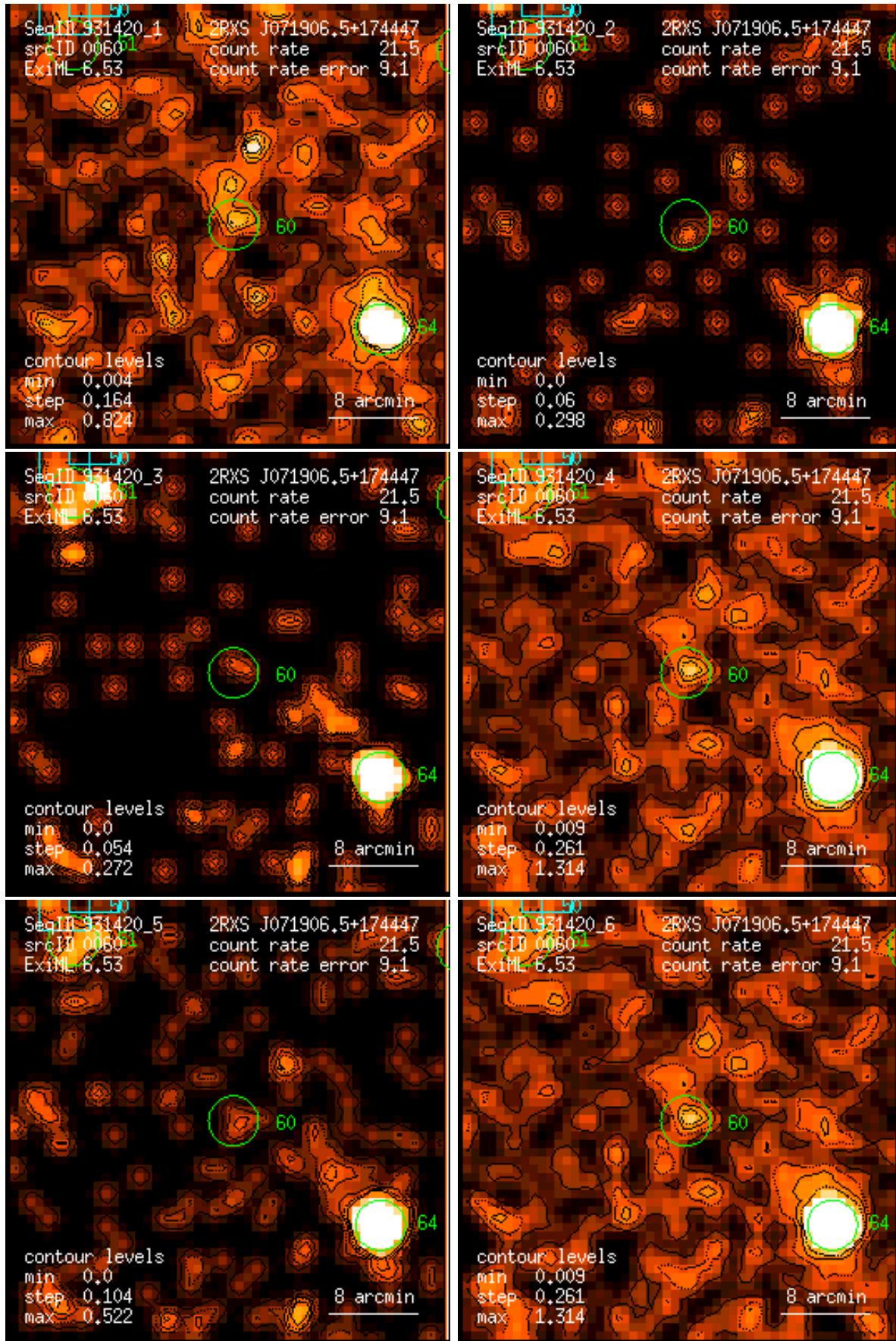
Figure 60: RASS 931420: detection 0060: band rate images, Gaussian filter: (1) PSPC channels 11 – 41, (2) 52 – 90, (3) 91 – 201, (4) 11 – 235, (5) 52 – 201, (6) 11 – 201. Broad band rates in counts/ks. Band rate contour levels in counts/ks/arcmin 2 .
