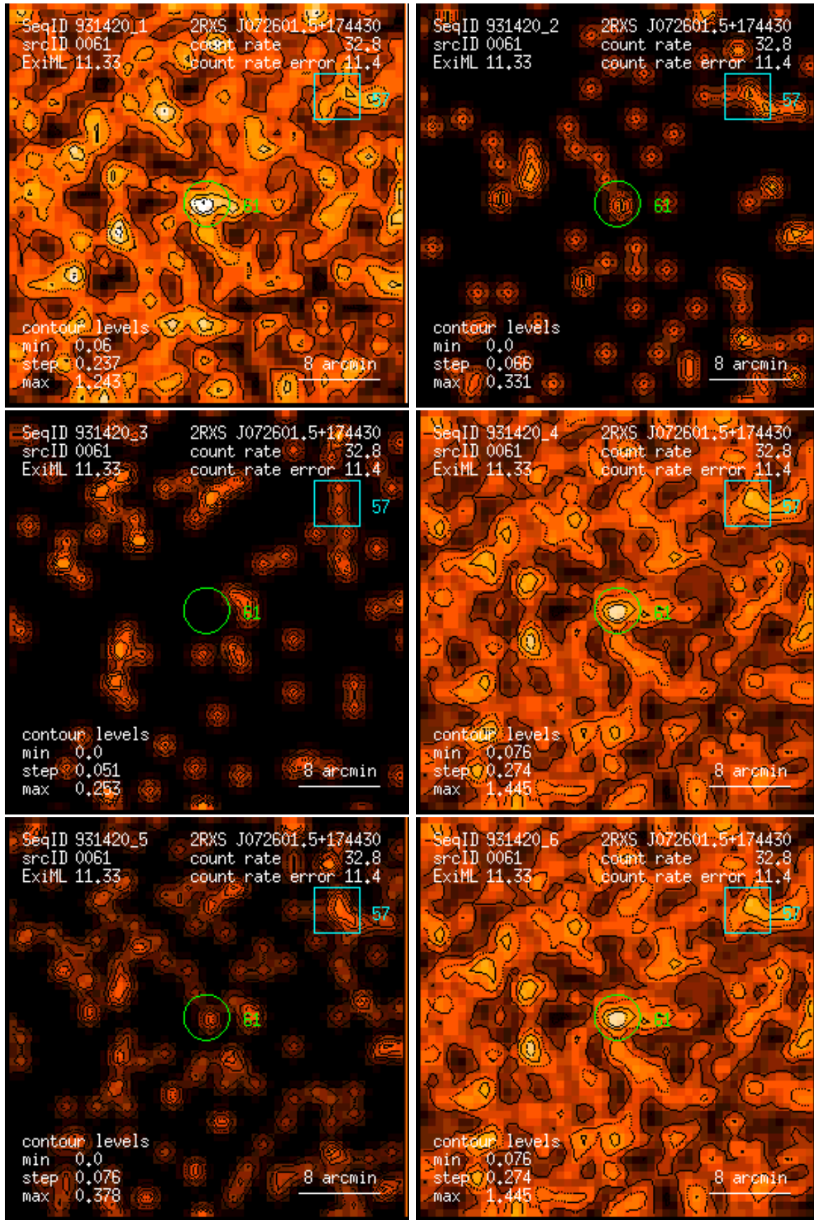
Figure 61: RASS 931420: detection 0061: band rate images, Gaussian filter: (1) PSPC channels 11 – 41, (2) 52 – 90, (3) 91 – 201, (4) 11 – 235, (5) 52 – 201, (6) 11 – 201. Broad band rates in counts/ks. Band rate contour levels in counts/ks/arcmin 2 .
