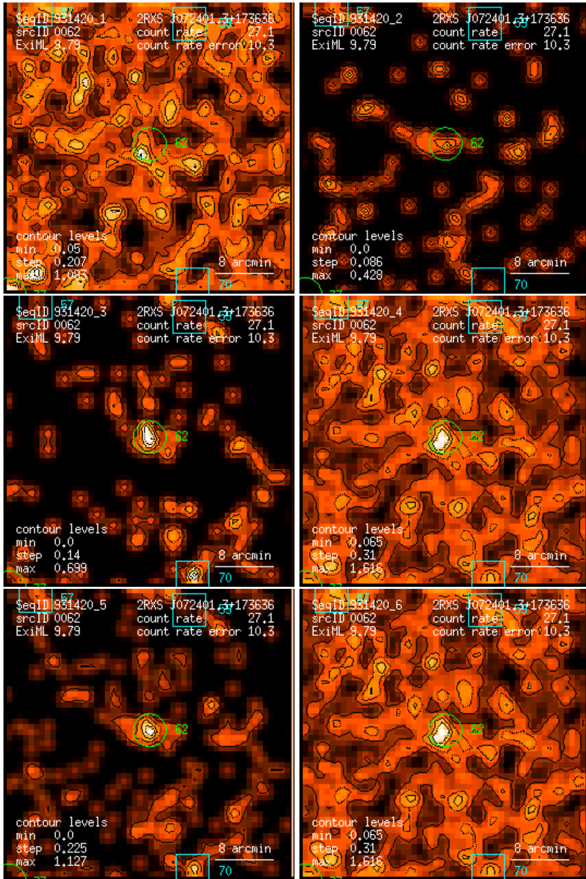
Figure 62: RASS 931420: detection 0062: band rate images, Gaussian filter: (1) PSPC channels 11 – 41, (2) 52 – 90, (3) 91 – 201, (4) 11 – 235, (5) 52 – 201, (6) 11 – 201. Broad band rates in counts/ks. Band rate contour levels in counts/ks/arcmin 2 .
