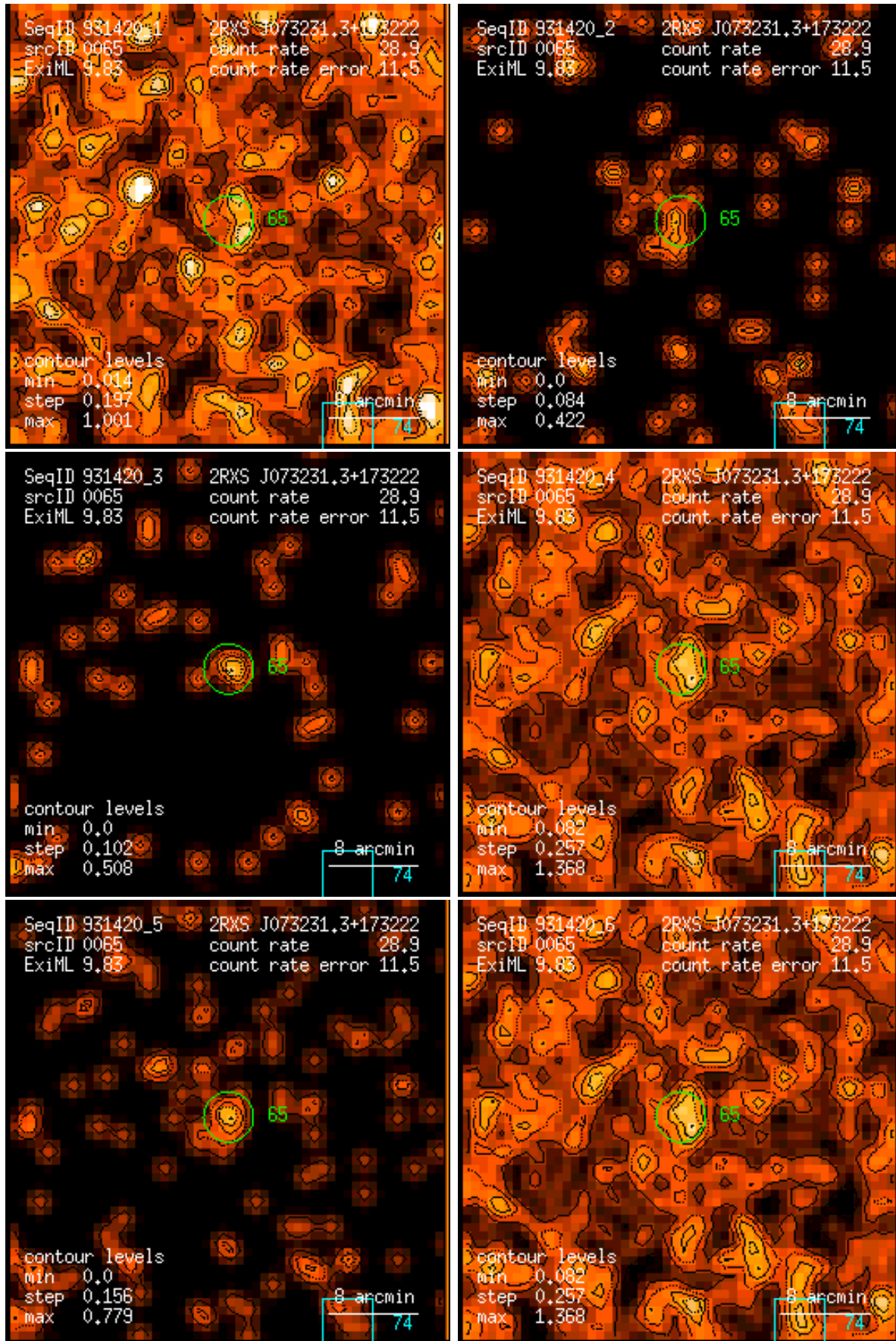
Figure 65: RASS 931420: detection 0065: band rate images, Gaussian filter: (1) PSPC channels 11 – 41, (2) 52 – 90, (3) 91 – 201, (4) 11 – 235, (5) 52 – 201, (6) 11 – 201. Broad band rates in counts/ks. Band rate contour levels in counts/ks/arcmin 2 .
