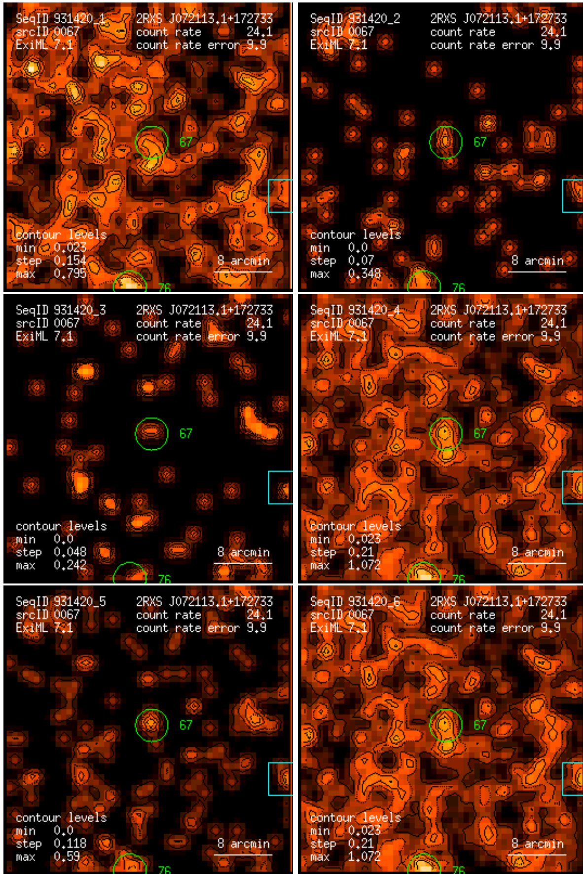
Figure 67: RASS 931420: detection 0067: band rate images, Gaussian filter: (1) PSPC channels 11 – 41, (2) 52 – 90, (3) 91 – 201, (4) 11 – 235, (5) 52 – 201, (6) 11 – 201. Broad band rates in counts/ks. Band rate contour levels in counts/ks/arcmin 2 .
