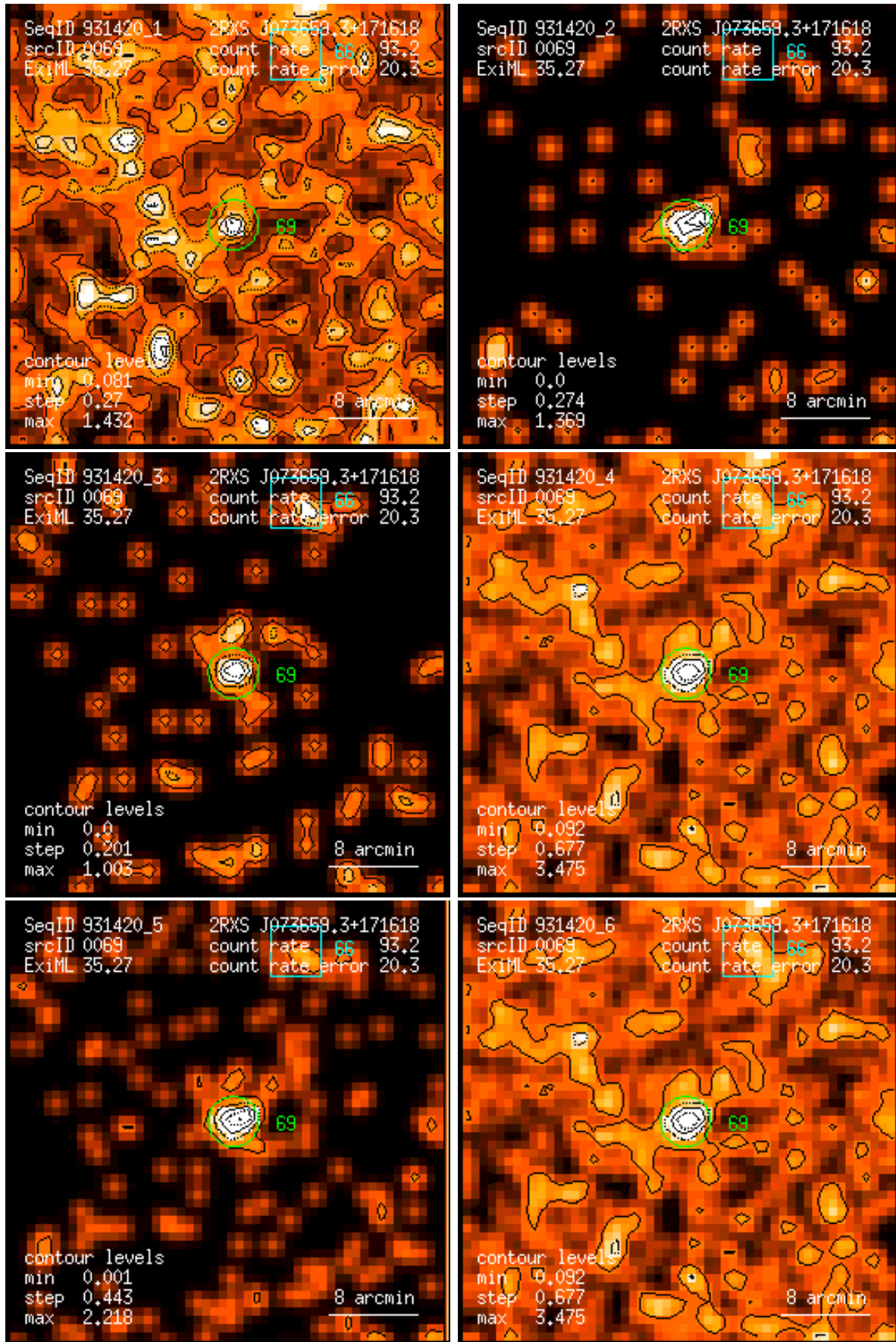
Figure 69: RASS 931420: detection 0069: band rate images, Gaussian filter: (1) PSPC channels 11 – 41, (2) 52 – 90, (3) 91 – 201, (4) 11 – 235, (5) 52 – 201, (6) 11 – 201. Broad band rates in counts/ks. Band rate contour levels in counts/ks/arcmin 2 .
