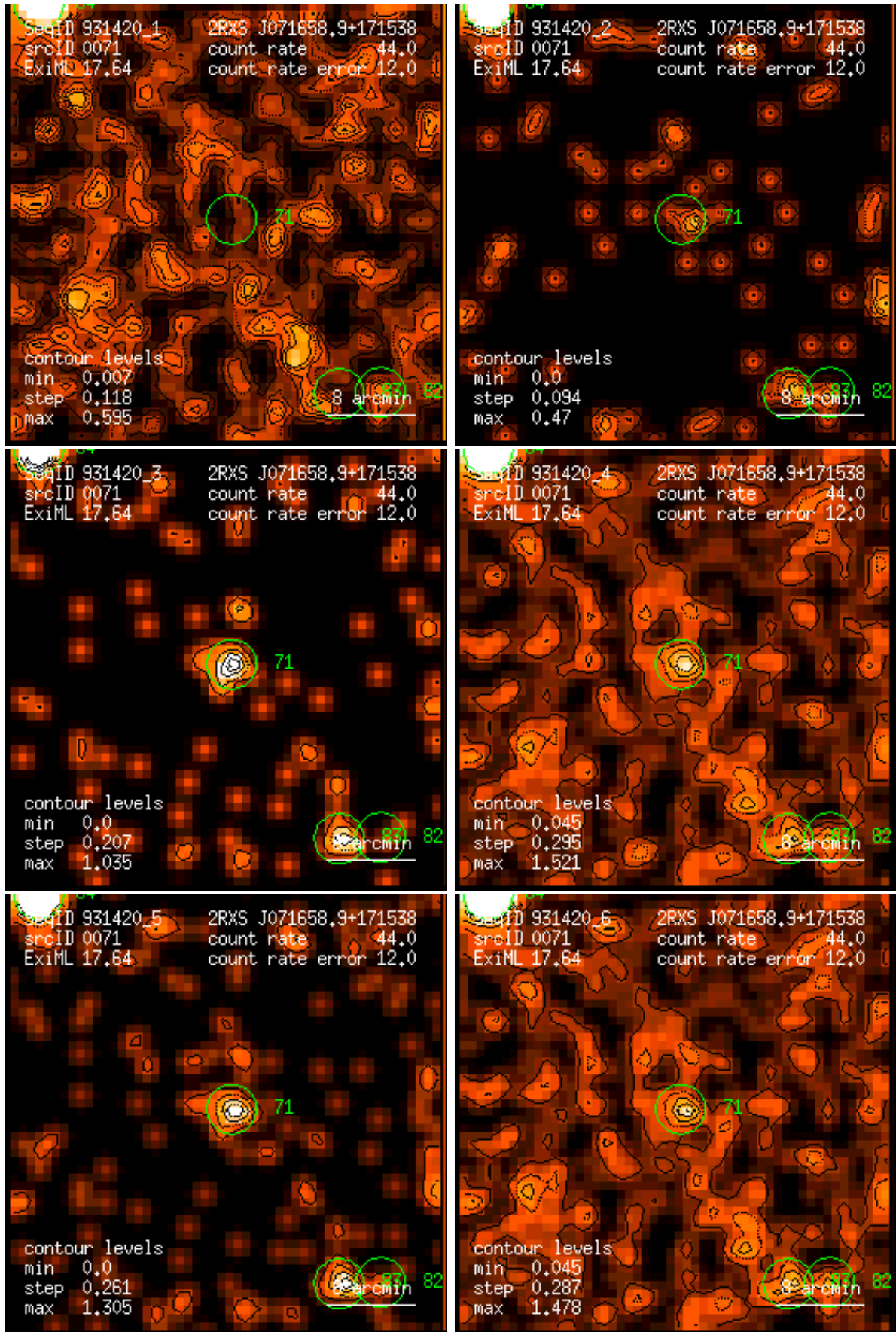
Figure 71: RASS 931420: detection 0071: band rate images, Gaussian filter: (1) PSPC channels 11 – 41, (2) 52 – 90, (3) 91 – 201, (4) 11 – 235, (5) 52 – 201, (6) 11 – 201. Broad band rates in counts/ks. Band rate contour levels in counts/ks/arcmin 2 .
