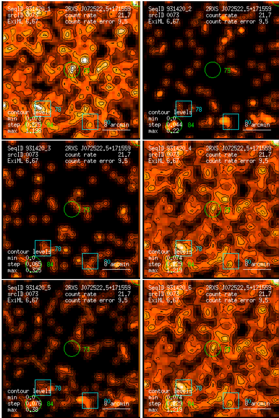
Figure 73: RASS 931420: detection 0073: band rate images, Gaussian filter: (1) PSPC channels 11 – 41, (2) 52 – 90, (3) 91 – 201, (4) 11 – 235, (5) 52 – 201, (6) 11 – 201. Broad band rates in counts/ks. Band rate contour levels in counts/ks/arcmin 2 .
