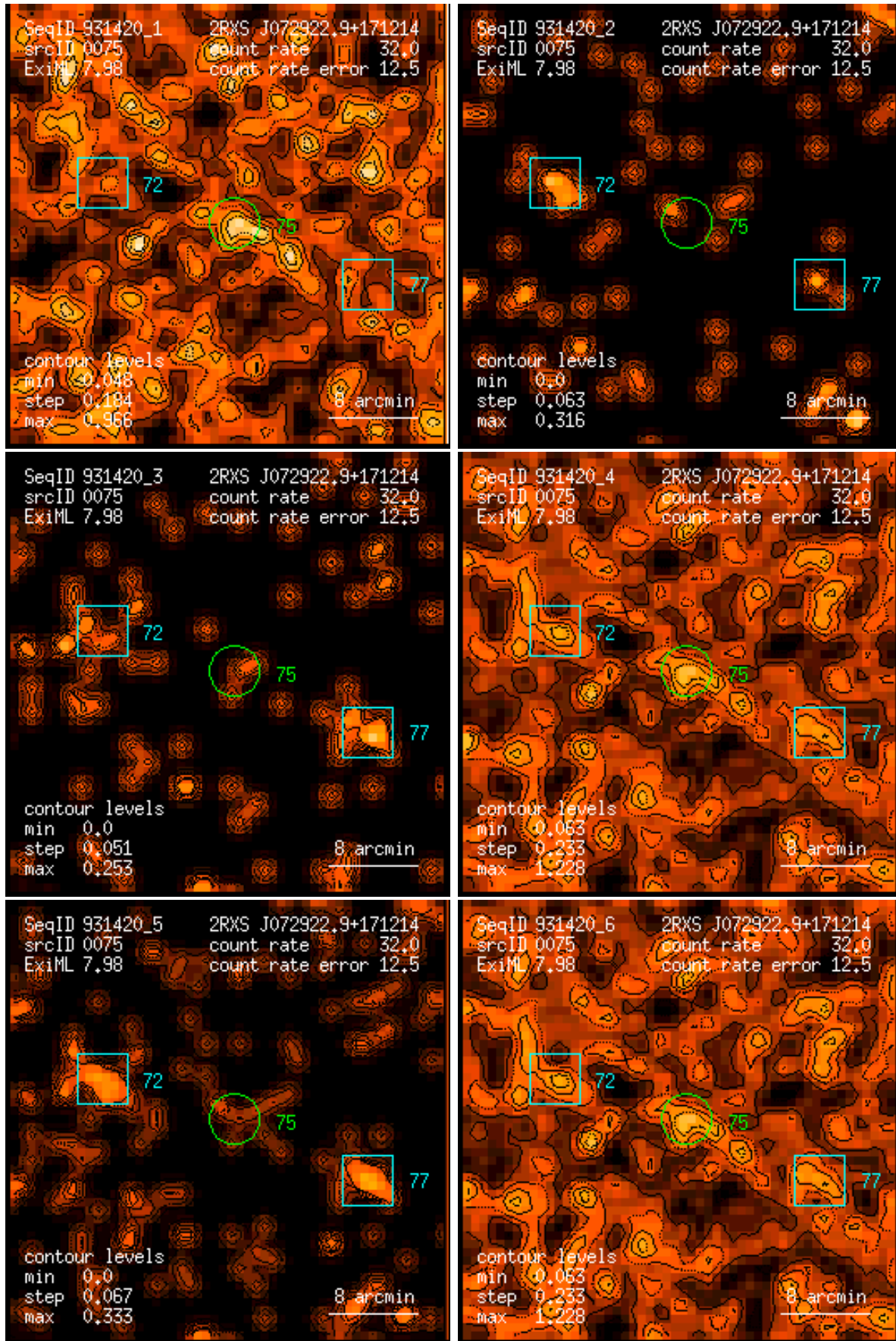
Figure 75: RASS 931420: detection 0075: band rate images, Gaussian filter: (1) PSPC channels 11 – 41, (2) 52 – 90, (3) 91 – 201, (4) 11 – 235, (5) 52 – 201, (6) 11 – 201. Broad band rates in counts/ks. Band rate contour levels in counts/ks/arcmin 2 .
