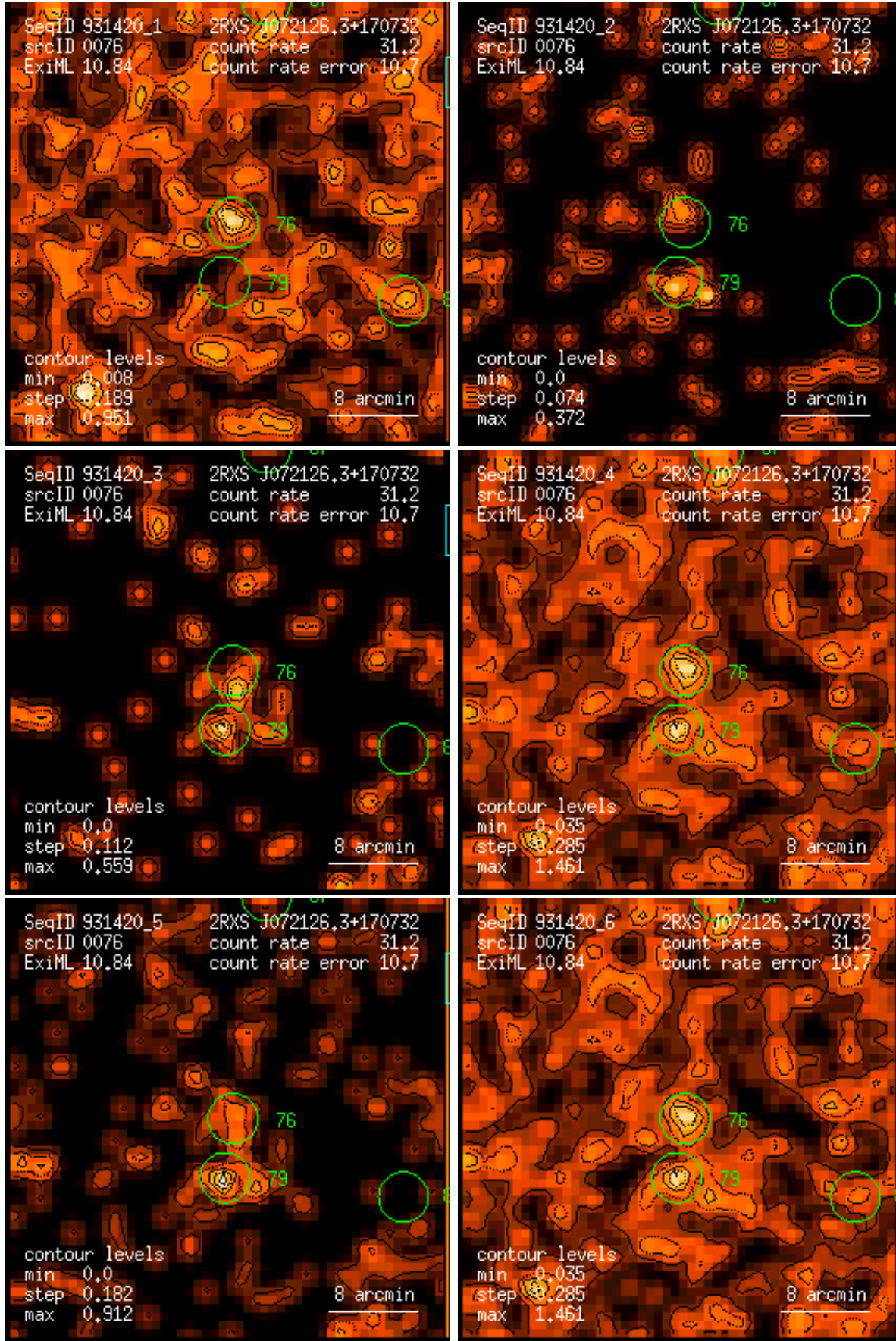
Figure 76: RASS 931420: detection 0076: band rate images, Gaussian filter: (1) PSPC channels 11 – 41, (2) 52 – 90, (3) 91 – 201, (4) 11 – 235, (5) 52 – 201, (6) 11 – 201. Broad band rates in counts/ks. Band rate contour levels in counts/ks/arcmin 2 .
