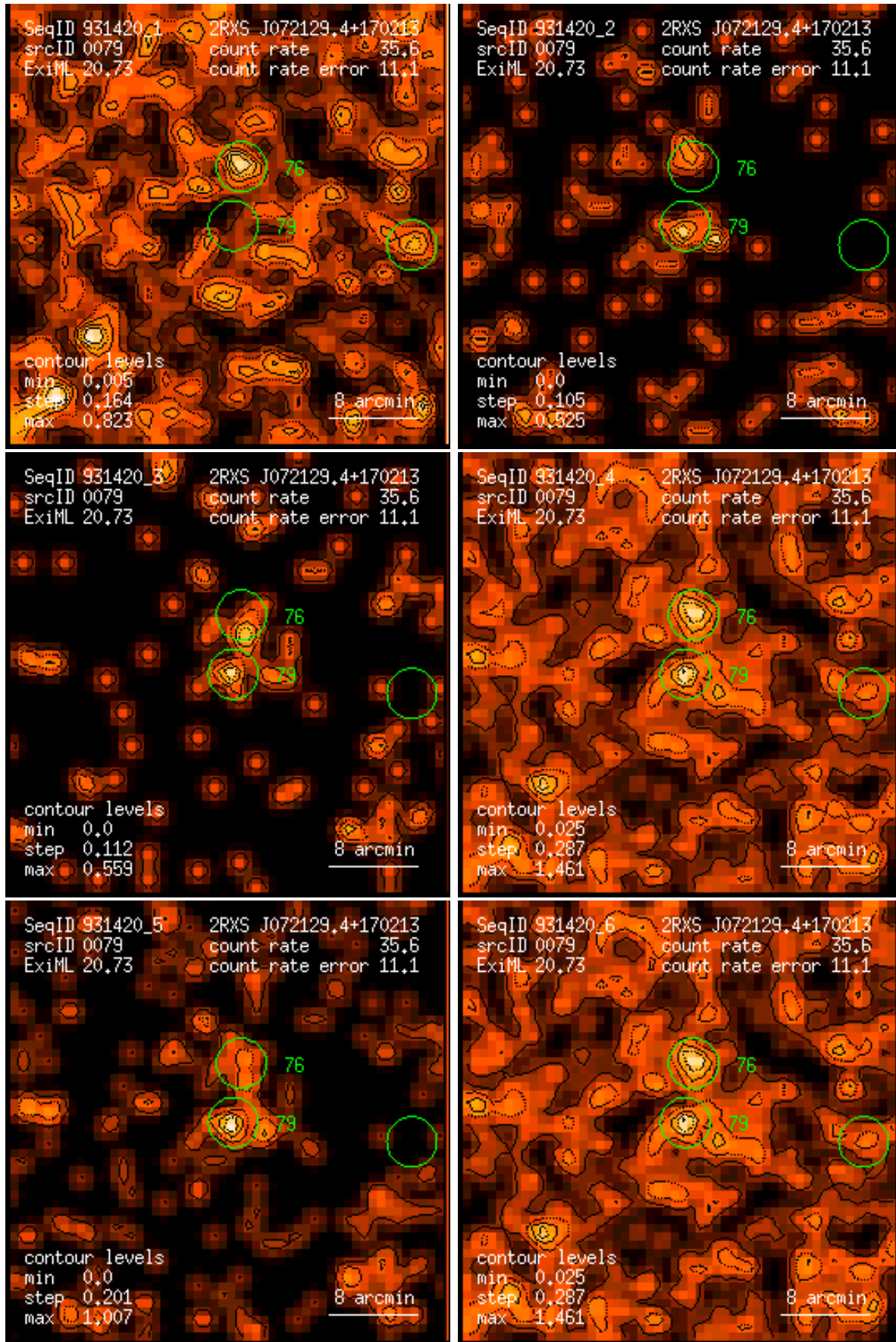
Figure 79: RASS 931420: detection 0079: band rate images, Gaussian filter: (1) PSPC channels 11 – 41, (2) 52 – 90, (3) 91 – 201, (4) 11 – 235, (5) 52 – 201, (6) 11 – 201. Broad band rates in counts/ks. Band rate contour levels in counts/ks/arcmin 2 .
