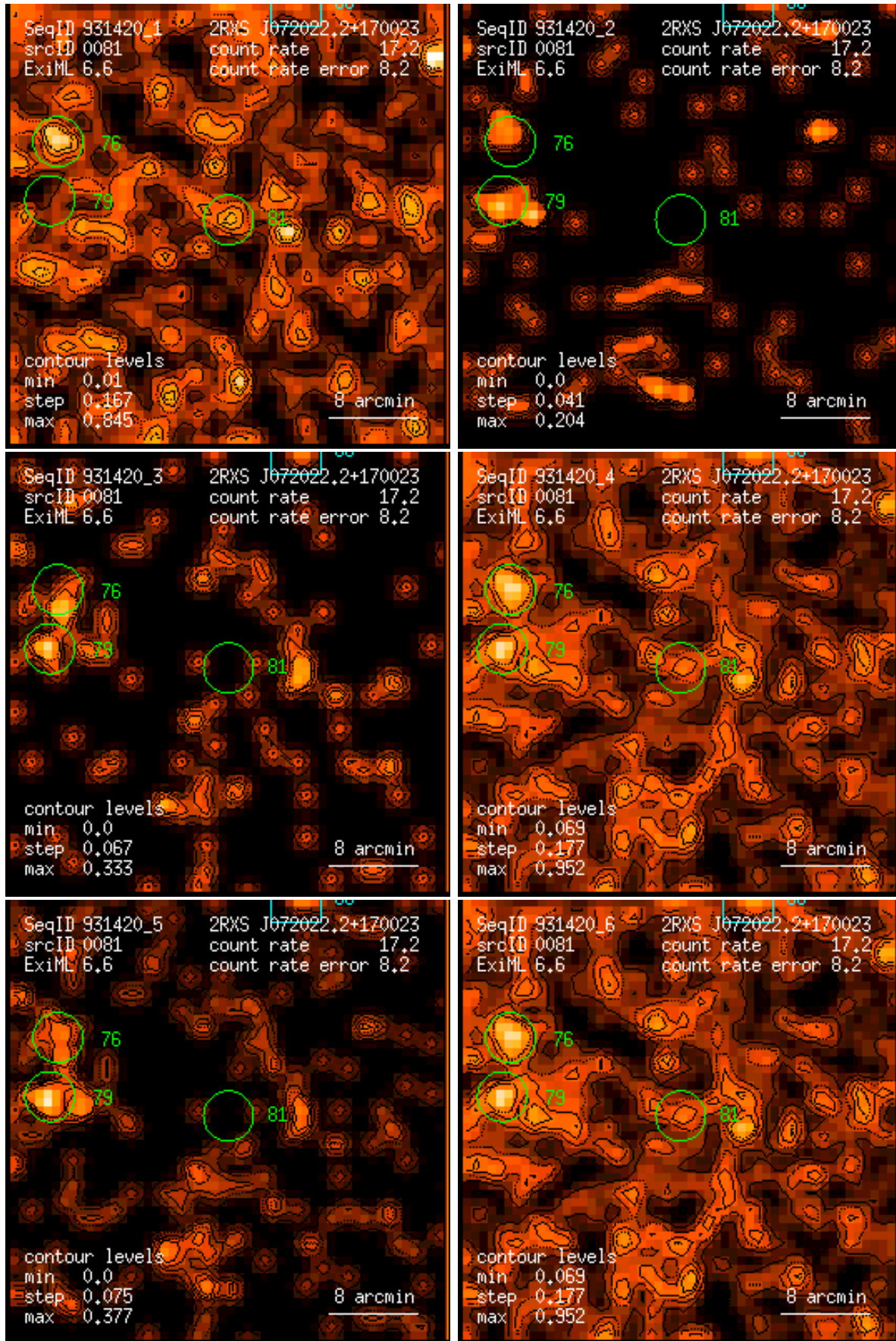
Figure 81: RASS 931420: detection 0081: band rate images, Gaussian filter: (1) PSPC channels 11 – 41, (2) 52 – 90, (3) 91 – 201, (4) 11 – 235, (5) 52 – 201, (6) 11 – 201. Broad band rates in counts/ks. Band rate contour levels in counts/ks/arcmin 2 .
