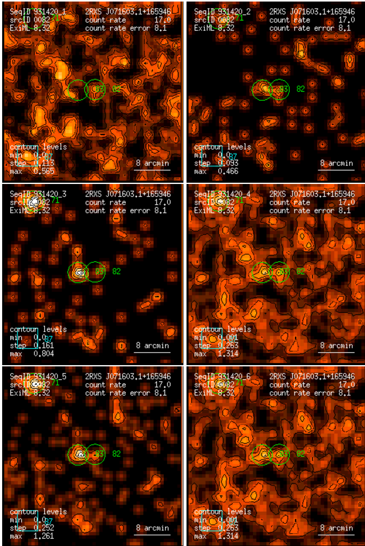
Figure 82: RASS 931420: detection 0082: band rate images, Gaussian filter: (1) PSPC channels 11 – 41, (2) 52 – 90, (3) 91 – 201, (4) 11 – 235, (5) 52 – 201, (6) 11 – 201. Broad band rates in counts/ks. Band rate contour levels in counts/ks/arcmin 2 .
