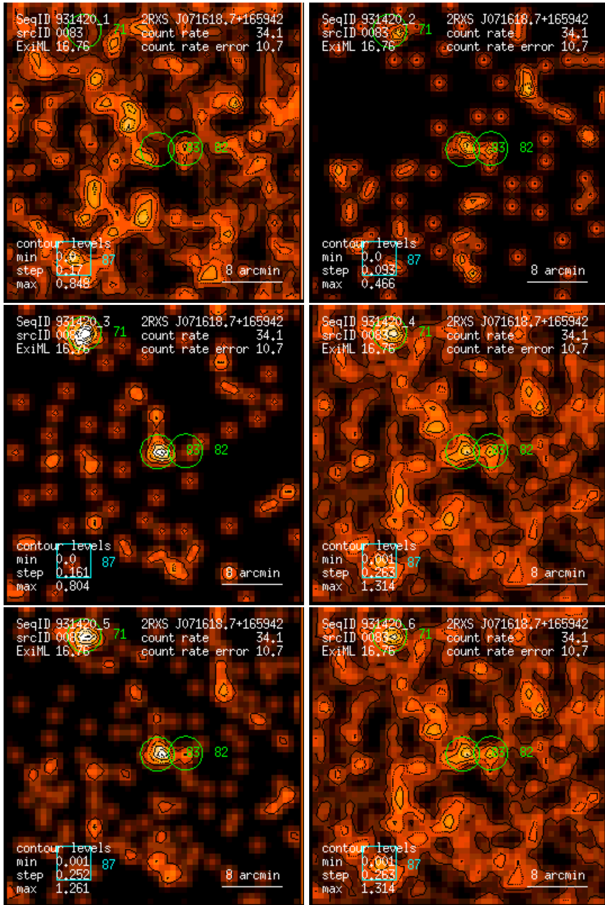
Figure 83: RASS 931420: detection 0083: band rate images, Gaussian filter: (1) PSPC channels 11 – 41, (2) 52 – 90, (3) 91 – 201, (4) 11 – 235, (5) 52 – 201, (6) 11 – 201. Broad band rates in counts/ks. Band rate contour levels in counts/ks/arcmin 2 .
