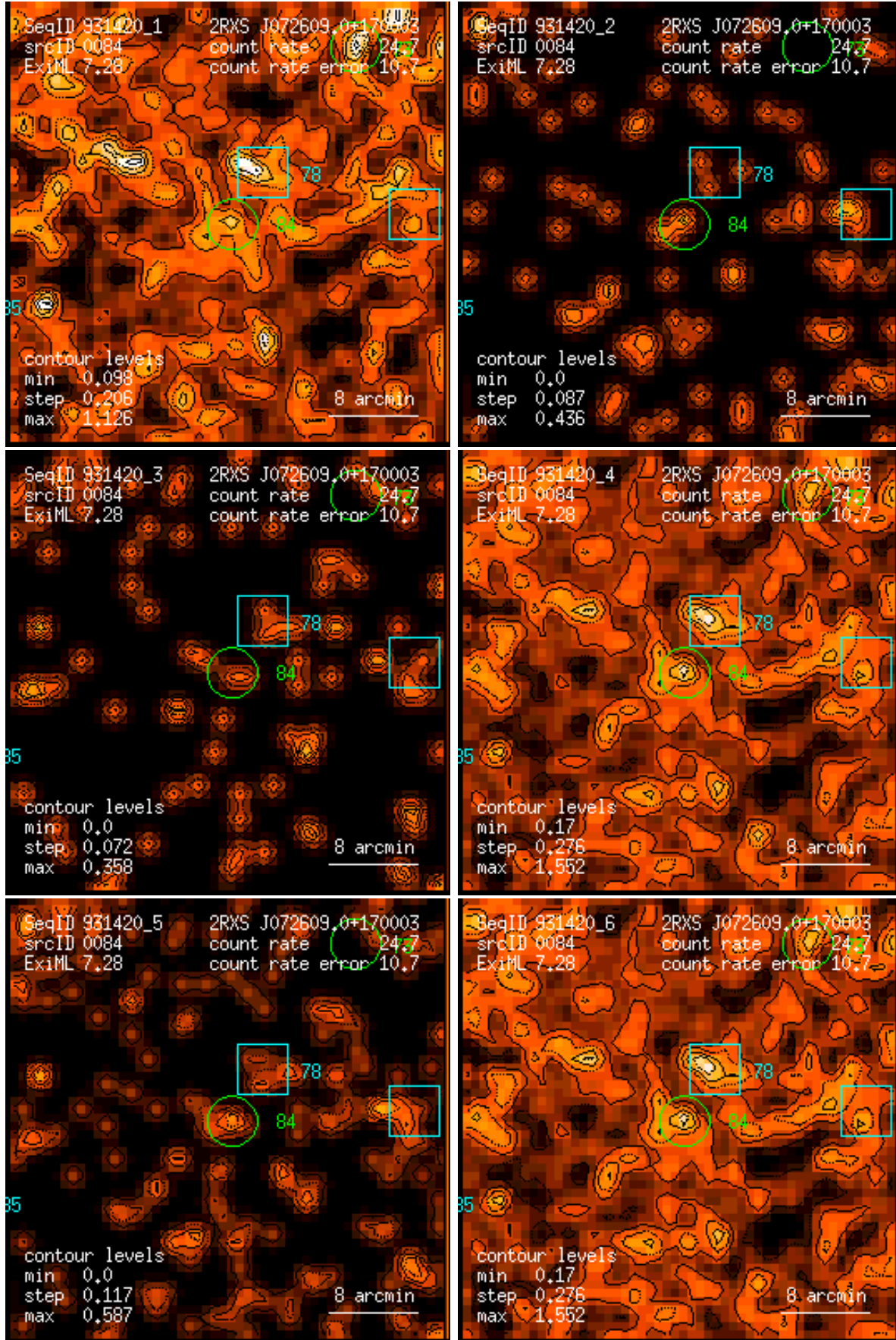
Figure 84: RASS 931420: detection 0084: band rate images, Gaussian filter: (1) PSPC channels 11 – 41, (2) 52 – 90, (3) 91 – 201, (4) 11 – 235, (5) 52 – 201, (6) 11 – 201. Broad band rates in counts/ks. Band rate contour levels in counts/ks/arcmin 2 .
