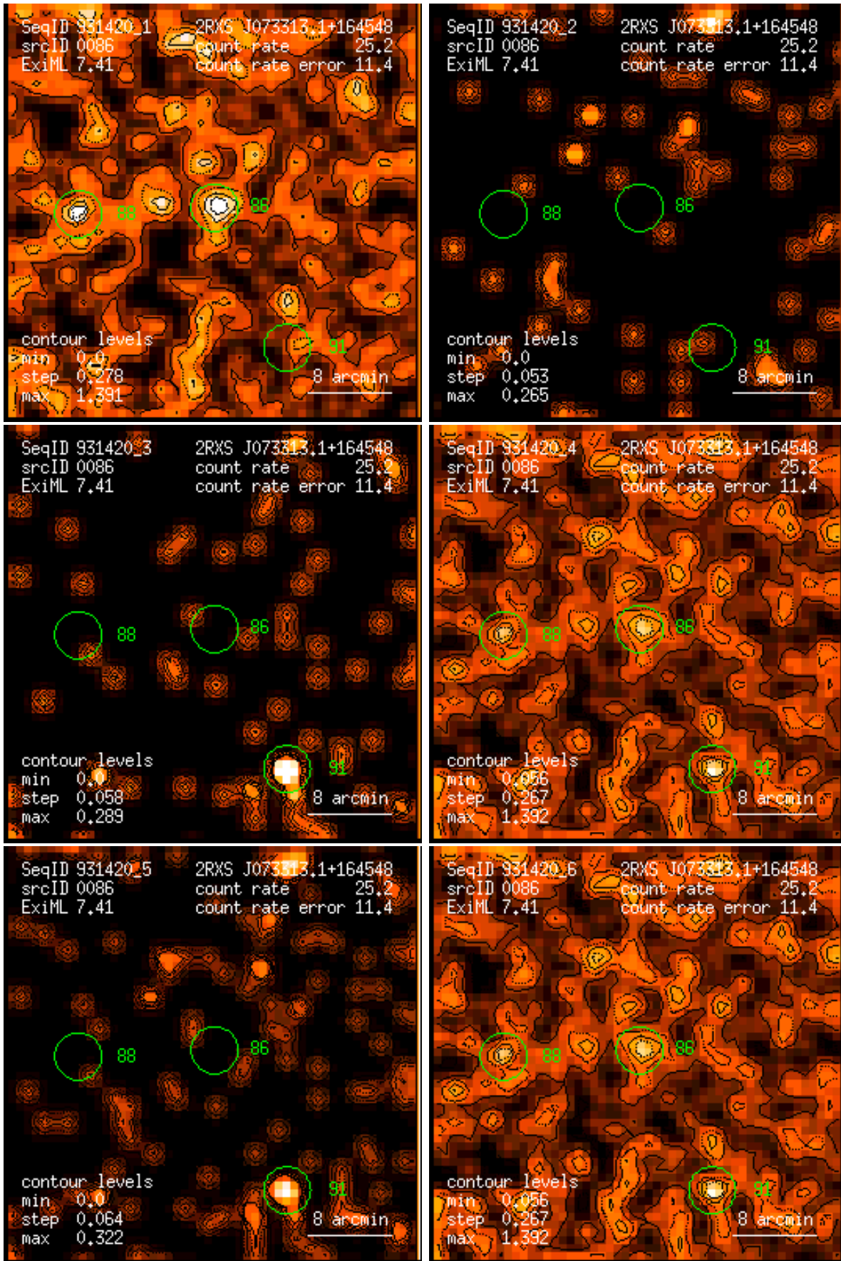
Figure 86: RASS 931420: detection 0086: band rate images, Gaussian filter: (1) PSPC channels 11 – 41, (2) 52 – 90, (3) 91 – 201, (4) 11 – 235, (5) 52 – 201, (6) 11 – 201. Broad band rates in counts/ks. Band rate contour levels in counts/ks/arcmin 2 .
