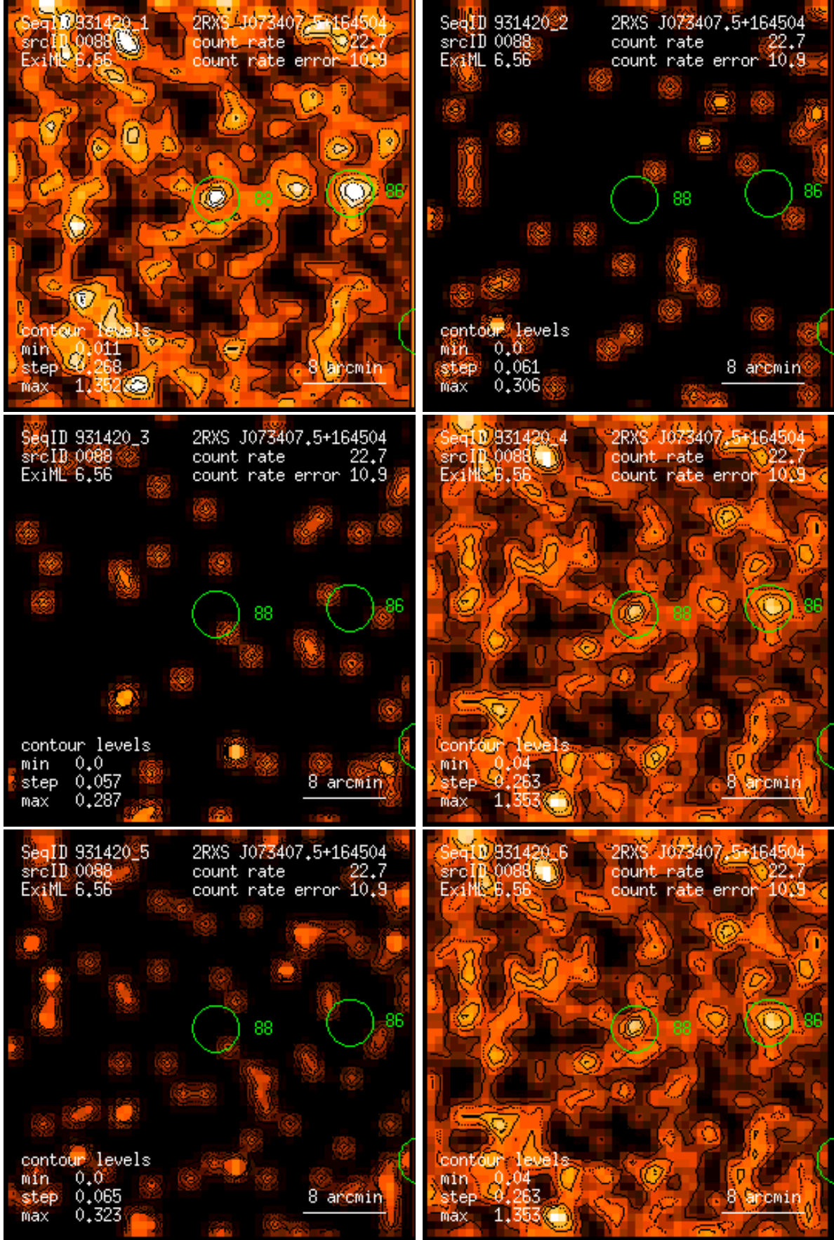
Figure 88: RASS 931420: detection 0088: band rate images, Gaussian filter: (1) PSPC channels 11 – 41, (2) 52 – 90, (3) 91 – 201, (4) 11 – 235, (5) 52 – 201, (6) 11 – 201. Broad band rates in counts/ks. Band rate contour levels in counts/ks/arcmin 2 .
